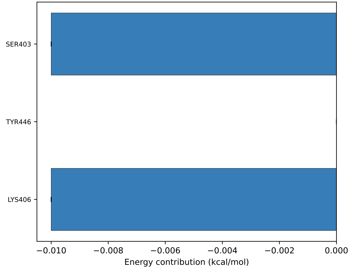
ALL_QU04: \Delta G = -1687.2 kcal/mol
