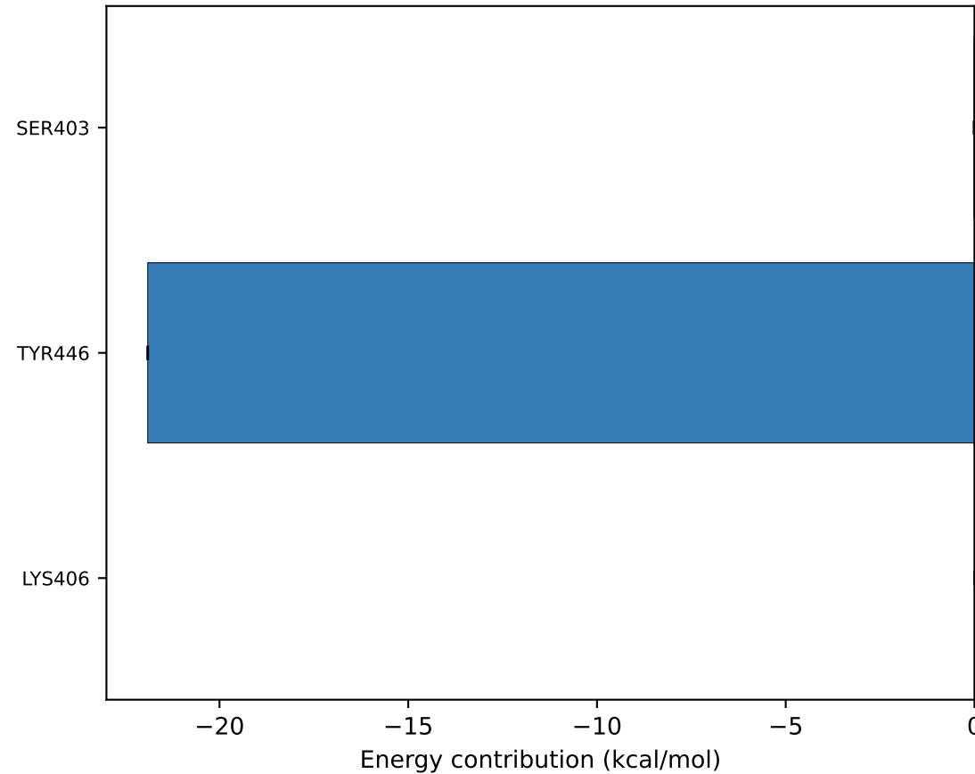
BRICS_0022: \Delta G = -523.5 kcal/mol
