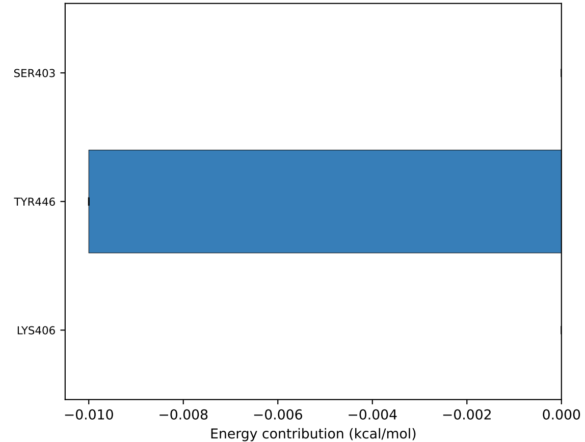
SEED_01150: \Delta G = -29.6 kcal/mol
