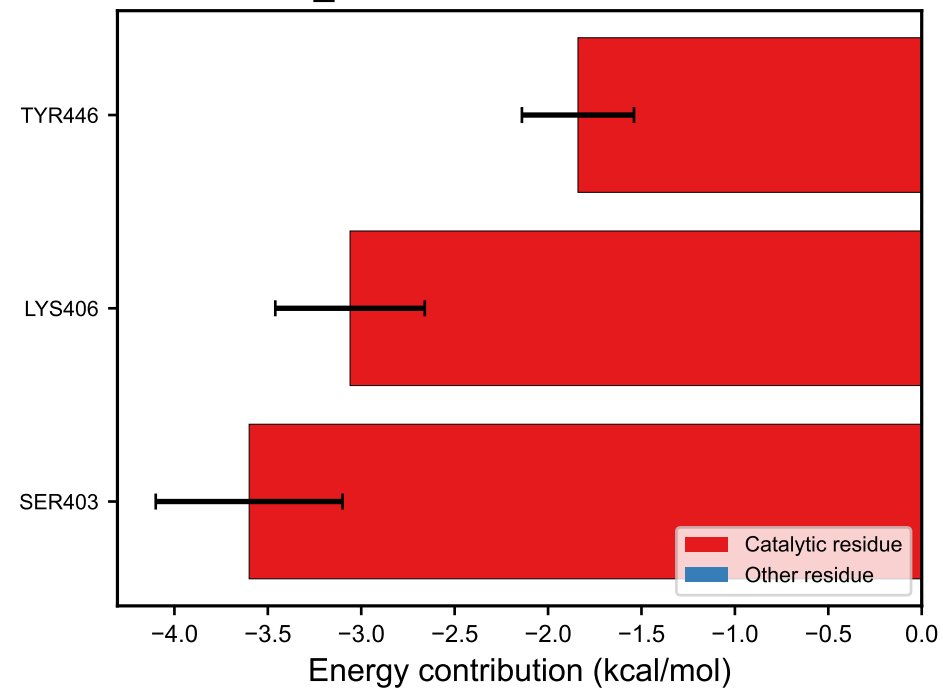
ALL_QU04: \Delta G = -34.4 kcal/mol
