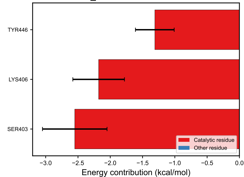
BRICS_0022: \Delta G = -20.4 kcal/mol
