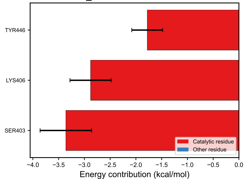
SEED_01150: \Delta G = -31.6 kcal/mol
