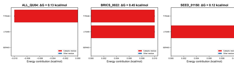
Figure 8: Per-residue MM-GBSA (OBC2) decomposition of the catalytic triad for the three candidates subjected to explicit-solvent MD, evaluated at the energy-minimised complex pose. All contributions are within \pm 0.1 kcal mol -1 . These small-magnitude per-residue contributions reflect the single energy-minimised pose used in the decomposition and should be interpreted cautiously, rather than as evidence that the ligands depart the pocket (the ligands instead remain bound over the short simulated MD).
