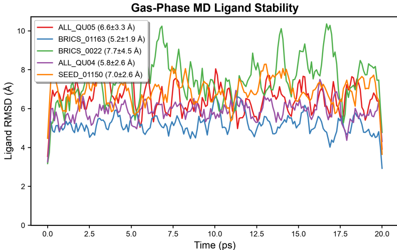
Figure 6: Ligand RMSD over explicit-solvent MD (100 ps NPT, TIP3P, 150 mM NaCl) for the top five candidates. None of the candidates reach a stable plateau within the simulation timescale.
