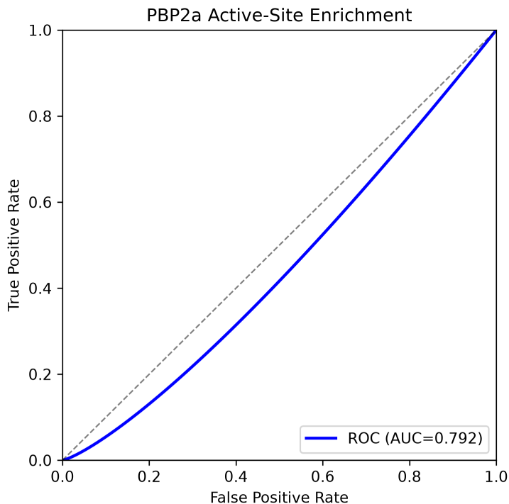
Figure 1: ROC curve for PBP2a enrichment validation. AUC = 0.792 , EF_{1\%} = 8.14 .
