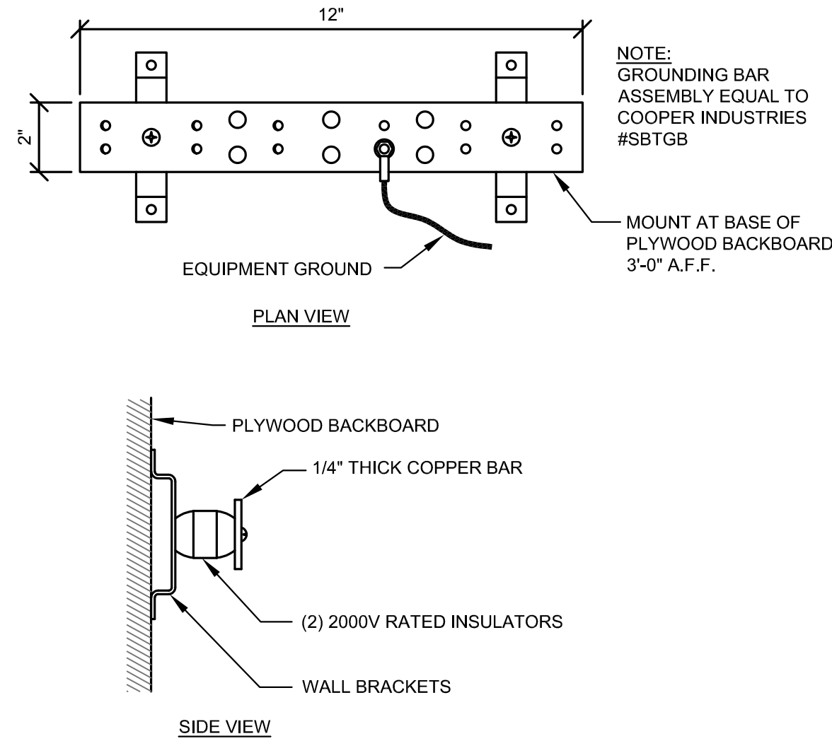
1 E5.1 N.T.S. TELECOMMUNICATIONS GROUNDING BAR DETAIL
