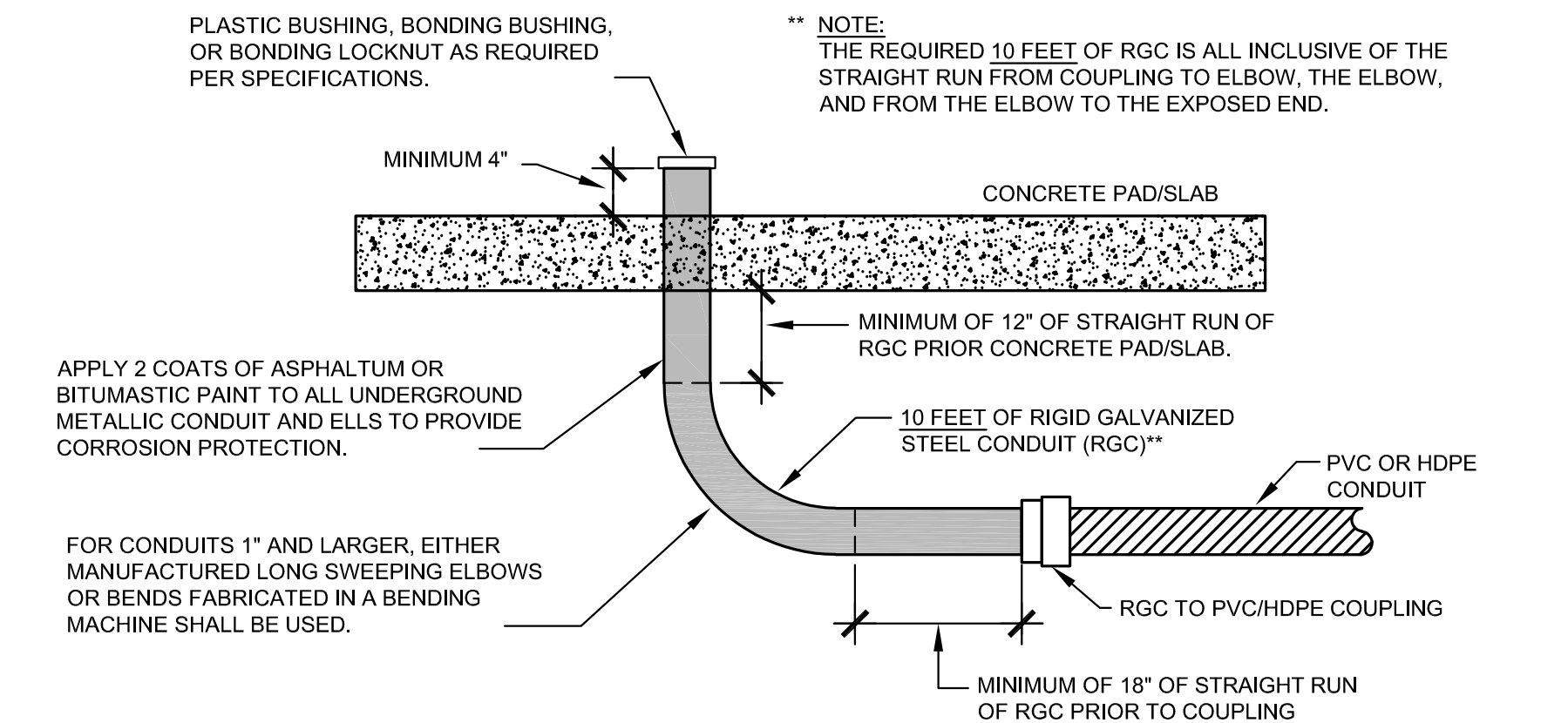
5 E5.1 N.T.S. CONDUIT STUB-UP DETAIL
