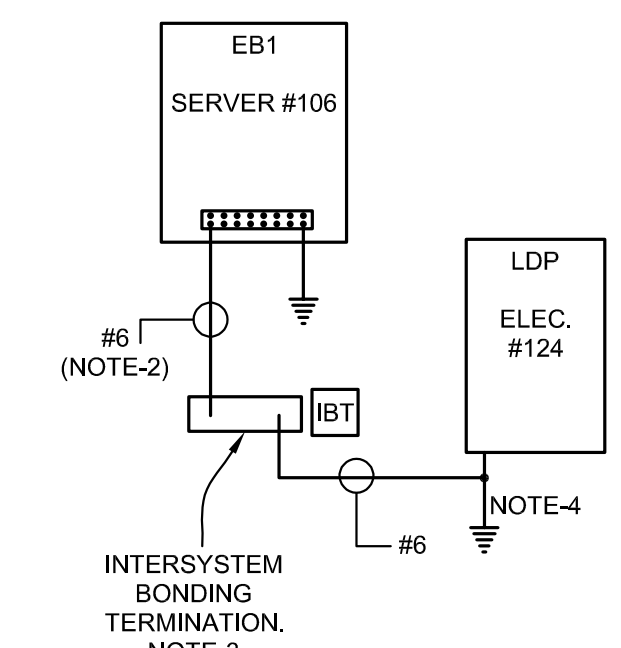
2 E5.1 N.T.S. TELECOMMUNICATIONS GROUNDING DETAIL
