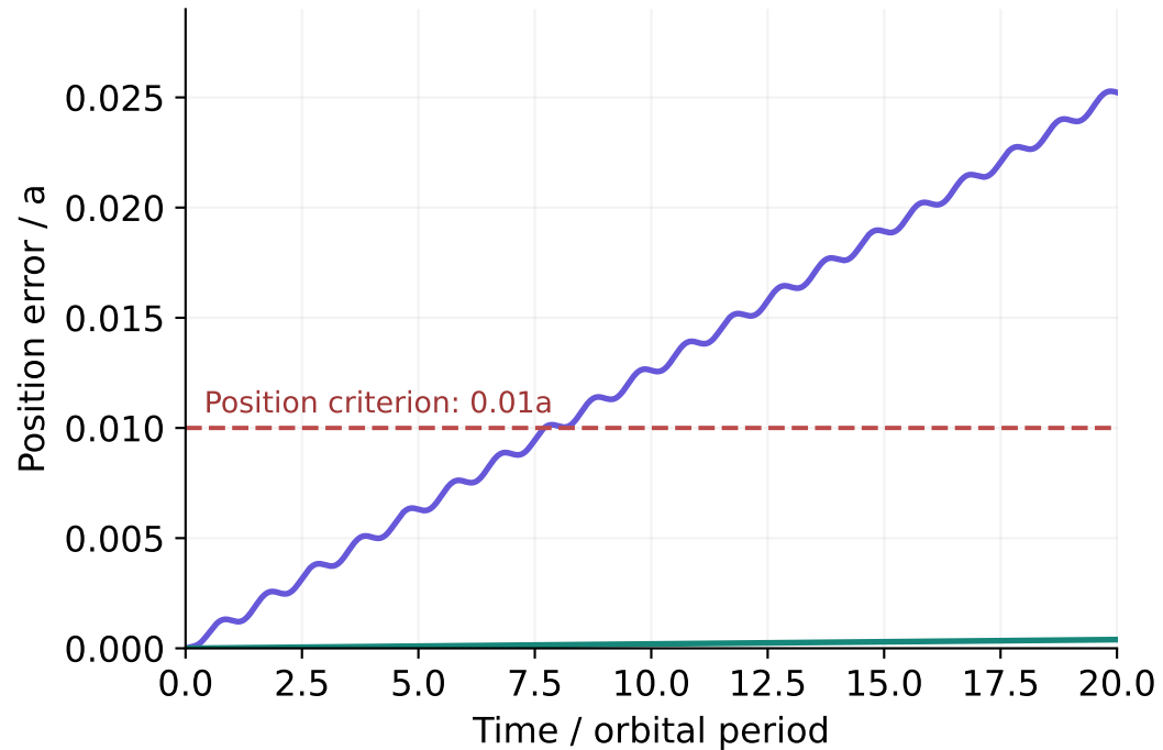
Position error exceeds the bound
