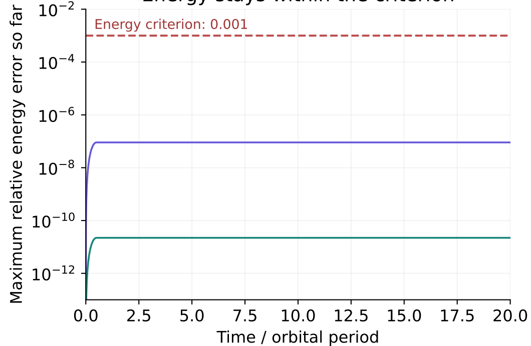
Energy stays within the criterion
