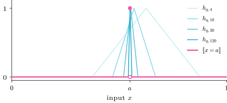
FIGURE 5. Tolerance tests h_{q,n} with q \rightarrow a and n \rightarrow \infty , chosen so that n|q - a| \rightarrow 0 , converge pointwise to the exact equality test \llbracket x = a \rrbracket , which is 1 at a and 0 elsewhere.
