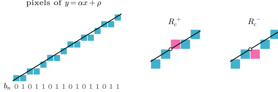
FIGURE 4. Left: the pixels drawn by Bresenham's algorithm for \alpha = (\sqrt{5} - 1)/2 , with the decision bits b_n . Right: where the line passes exactly through a pixel corner, the deep computations R_c^+ and R_c^- break the tie in opposite directions; they agree on every other pixel.
