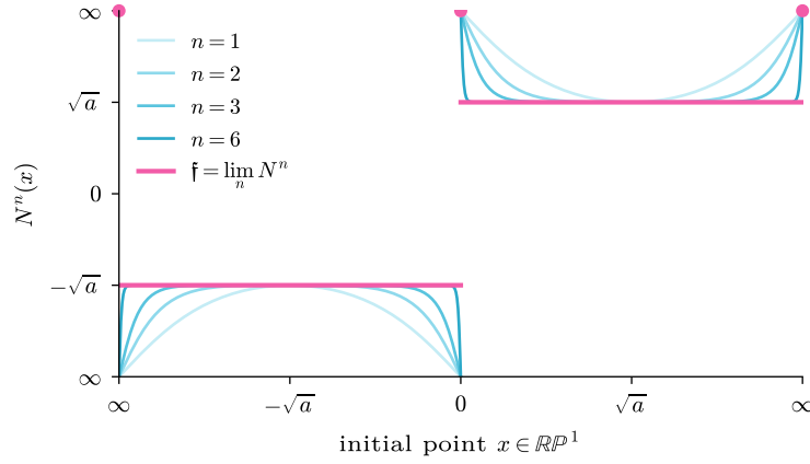
FIGURE 1. Newton iterates N_p^n for p(x) = x^2 - a on the real projective line, drawn on the circle with \infty at both ends of each axis. The continuous maps N_p^n converge pointwise to the deep computation \mathbf{f} , which sends the positive half line to \sqrt{a} , the negative half line to -\sqrt{a} , and 0 and \infty to \infty .
