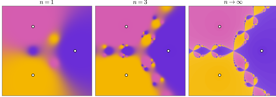
FIGURE 3. Newton's method for \kappa(z) = z^3 - 1 after one and three iterations, and its limit. The coloring blends the colors of the three cube roots of unity (white circles) according to the distance of N_\kappa^{(n)}(z) to each of them; the limit is constant on each basin and discontinuous across the Newton fractal; in the right panel, points are paler where convergence is slower.
