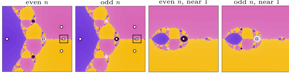
FIGURE 2. The deep computations of Newton's method for \rho(z) = z^3 - 2z + 2 : the limits of the even iterates N_\rho^{(2k)} and of the odd iterates N_\rho^{(2k+1)} , on the whole plane and near the point 1. Points in the basins of the real root and of the roots in the upper and lower half planes (white circles) are purple, orchid and gold, paler where convergence is slower. The remaining open region is the basin of the superattracting cycle 0 \mapsto 1 \mapsto 0 (white squares). A point there is lilac if the iterate in question is near 0 and plum if it is near 1, so the two colors exchange between even and odd iterates: the two deep computations agree on the basins of the roots and differ on the basin of the cycle. The boundaries of the colored regions form the Newton fractal of \rho .
