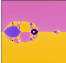
even n , near 1
