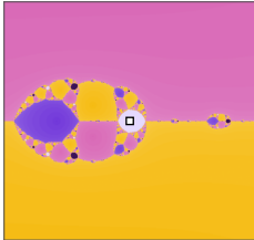
odd n , near 1
