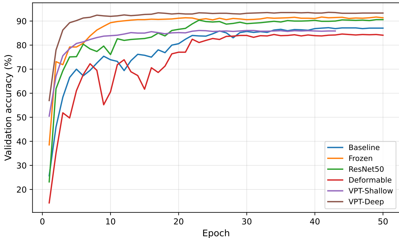
Training curves: validation accuracy per epoch
