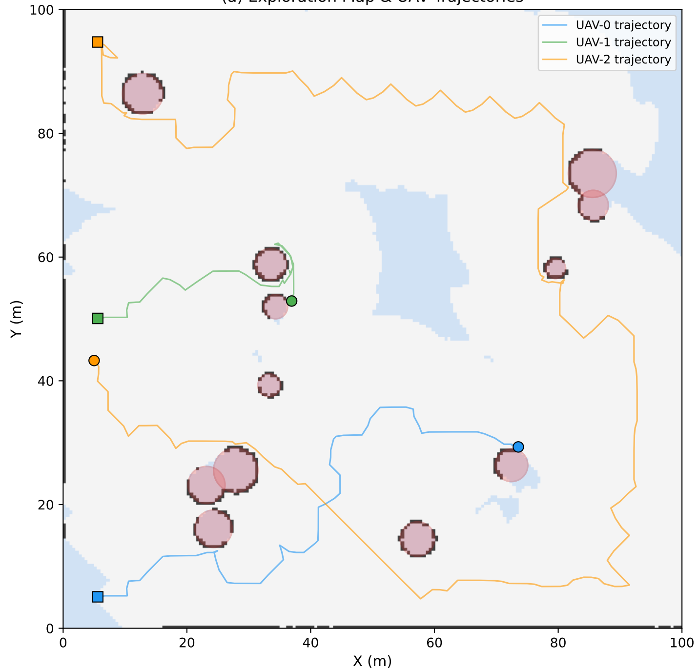
(a) Exploration Map & UAV Trajectories
