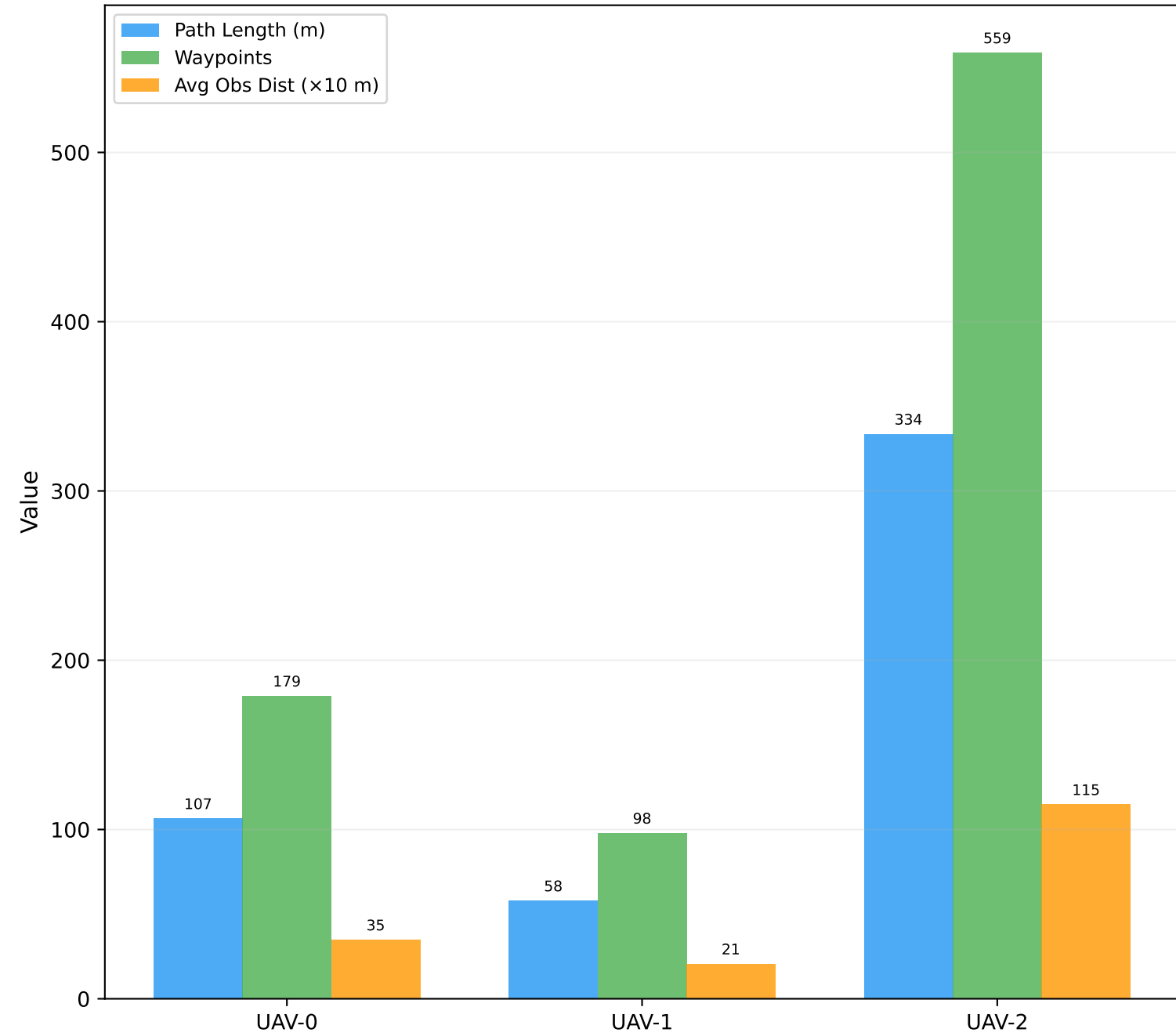
(b) Per-UAV Performance Metrics
