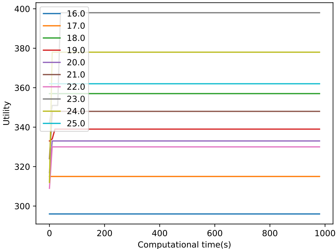
facebook AnytimeMCTS 1000
