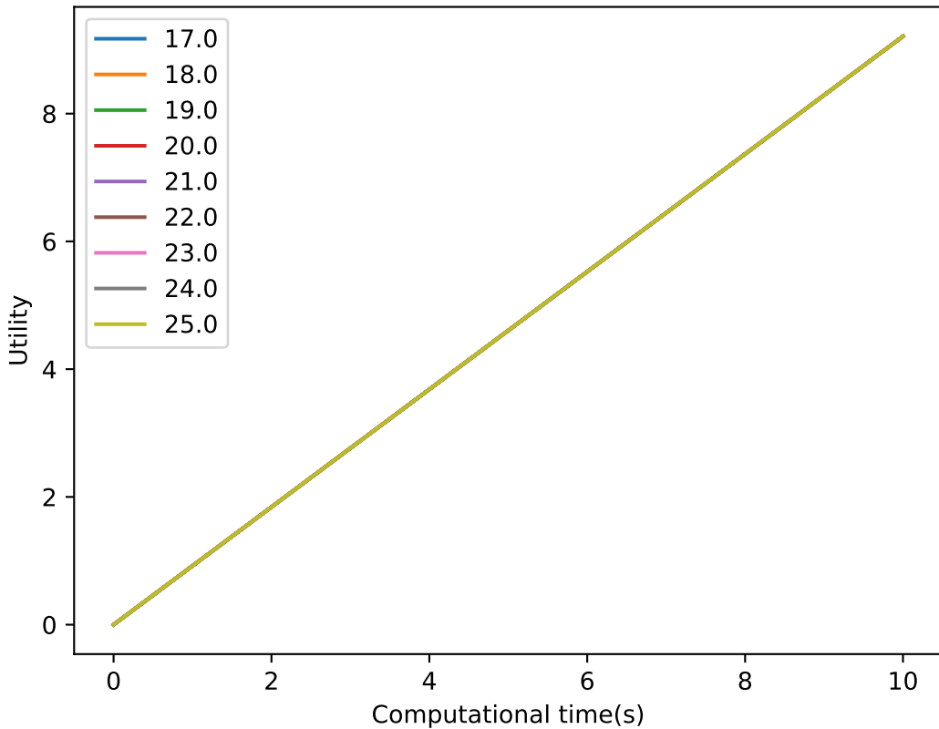
adult AnytimeEfficientBFS 111
