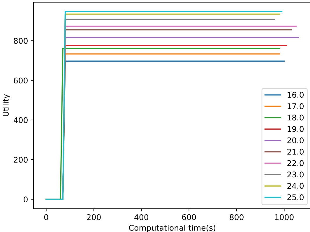
caltech AnytimeEfficient 767
