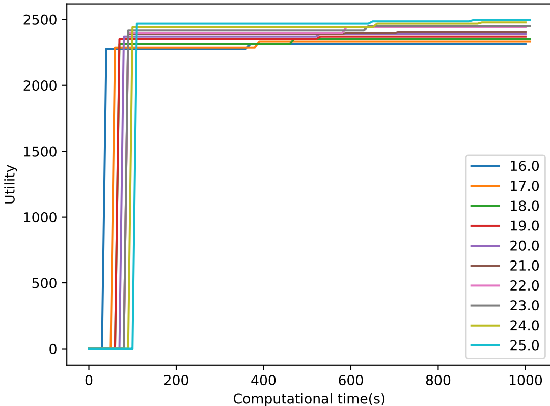
facebook AnytimeEfficientBFS 3000
