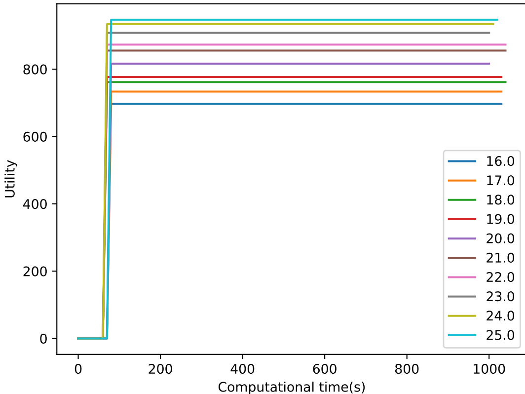
caltech AnytimeEfficientBFS 767
