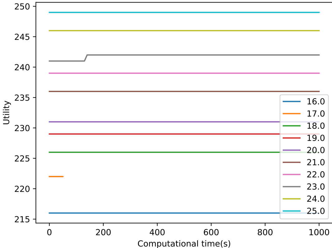
youtube AnytimeEfficientBFS 3000
