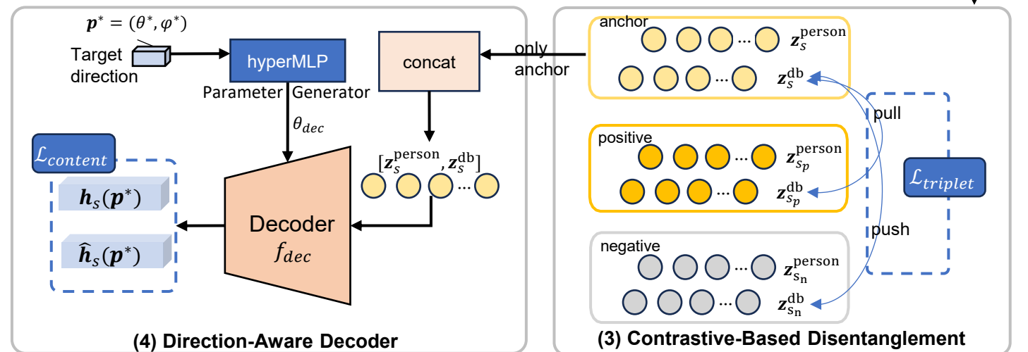
(b) Direction-Aware and Contrastive-Based Autoencoder
