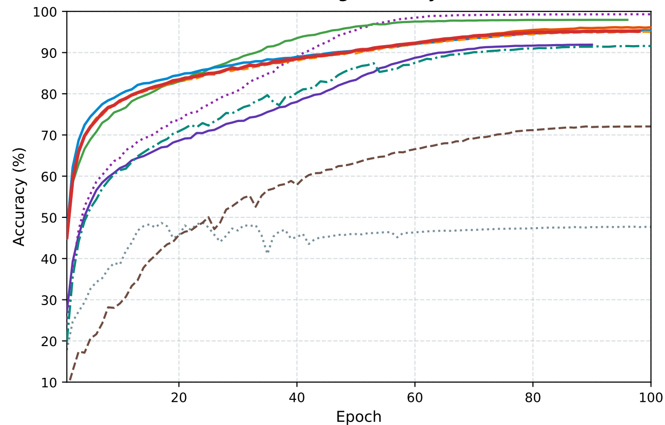
(b) Training Accuracy (%)
