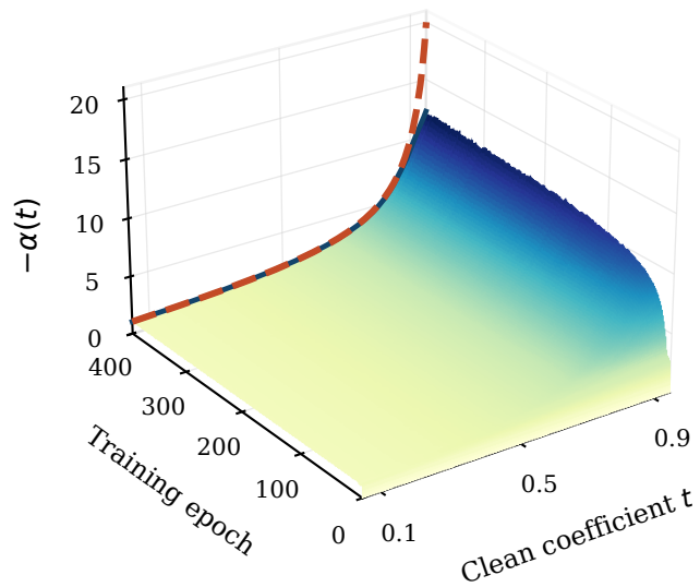
(a) Learned skip coefficient
