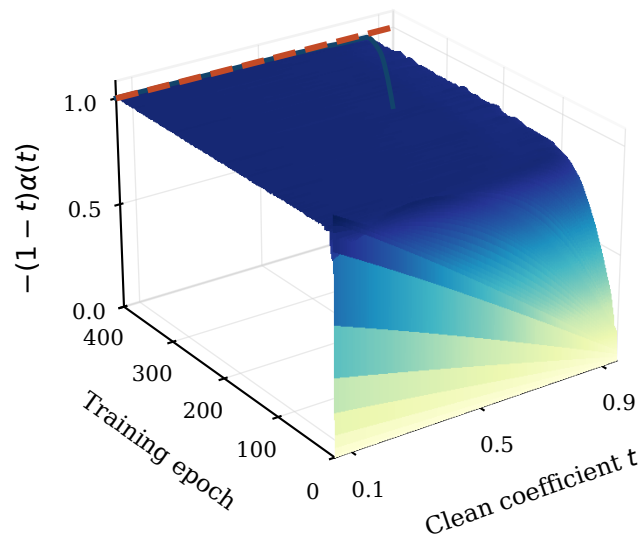
(b) Normalized skip coefficient
