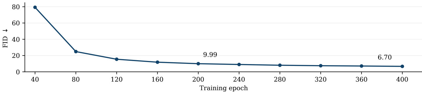
(c) Generation quality
