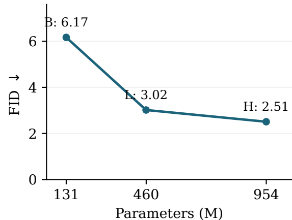
(a) Scaling at 200 epochs
