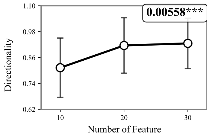
Metric
