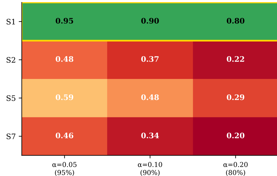
Raw similarity
