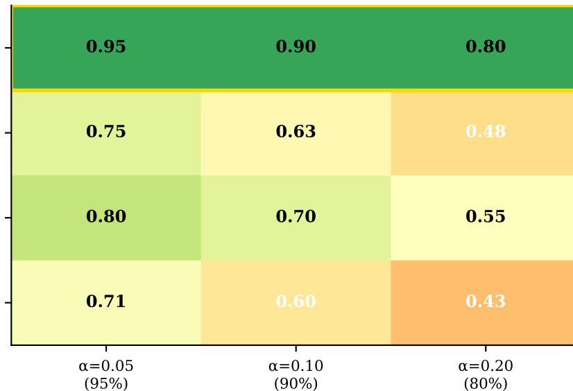
\kappa -modulated
