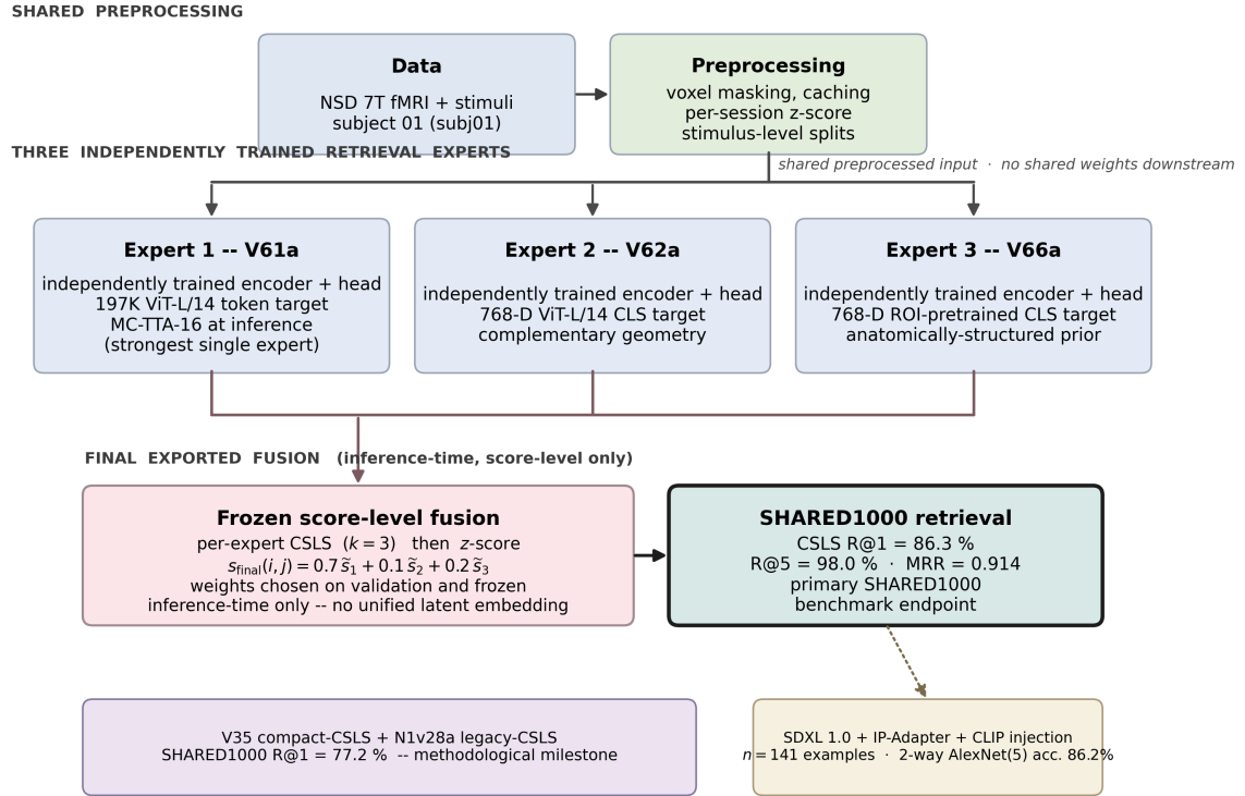
Figure 1.1: Overview of the complete thesis pipeline. NSD 7T fMRI from subject 01 passes through a single shared preprocessing stage and is then broadcast in parallel to three independently trained retrieval experts, V61a, V62a, and V66a, whose encoders and heads share no weights. At inference time, each expert produces a CSLS-corrected score matrix at neighbourhood size k = 3 ; the three score streams are z-score normalised per expert and combined by a frozen weighted sum with weights w_1/w_2/w_3 = 0.7/0.1/0.2 , yielding the primary SHARED1000 benchmark endpoint at 86.3% CSLS Recall@1 (heavy border). The fusion is applied at the retrieval-score level only and does not produce a unified fused latent embedding. The earlier V35 plus N1v28a fixed fusion at 77.2% is retained as a methodological milestone. The reconstruction add-on uses SDXL 1.0 with IP-Adapter visual conditioning anchored on the retrieved top-1 image plus fMRI-predicted CLIP injection, evaluated on 141 SHARED1000 examples.
