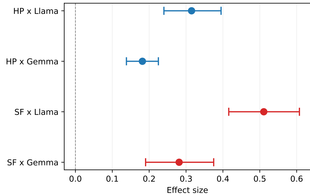
Retrieval Effect (REAL - SHUFFLED)
