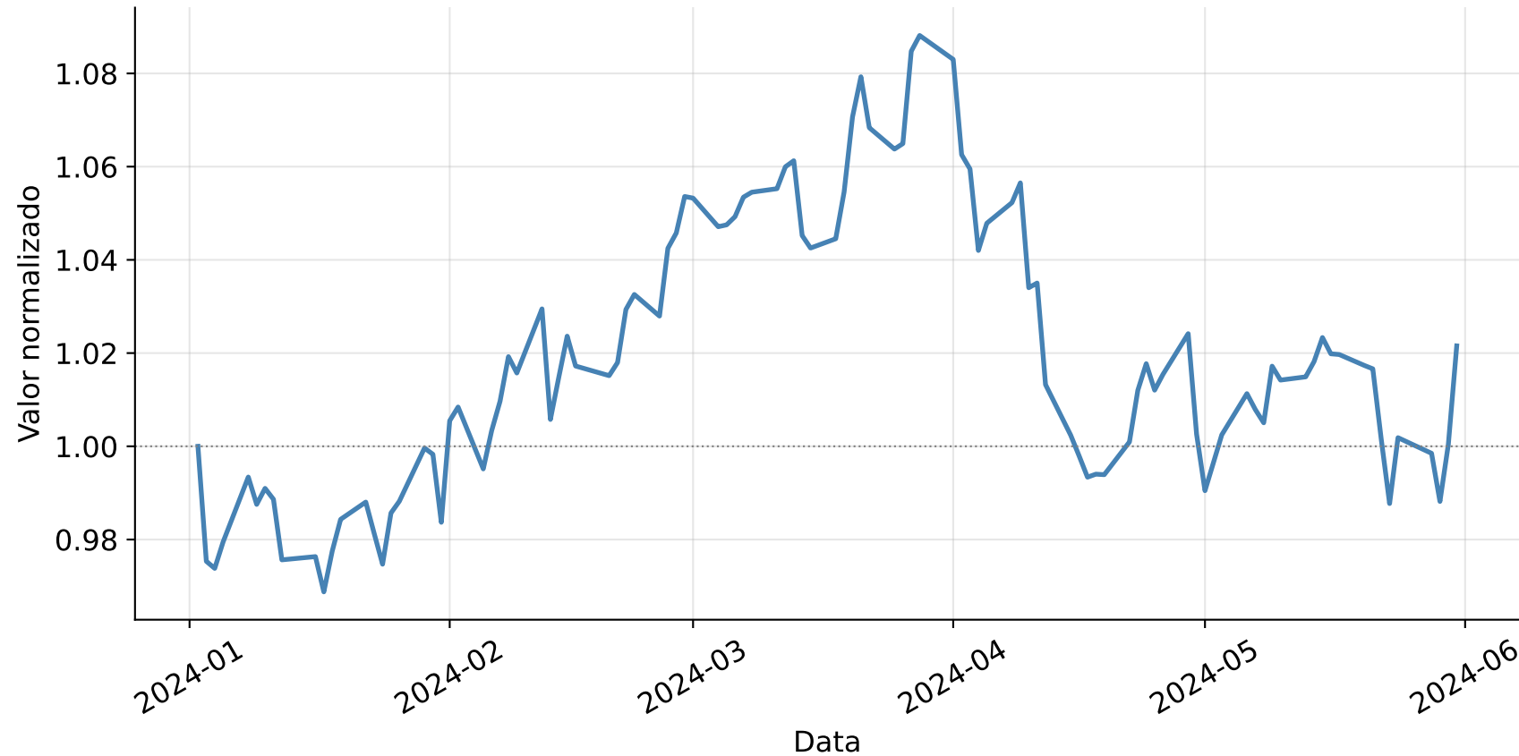
CONSUMER CYCLICALS — Performance OOS (normalizado)
