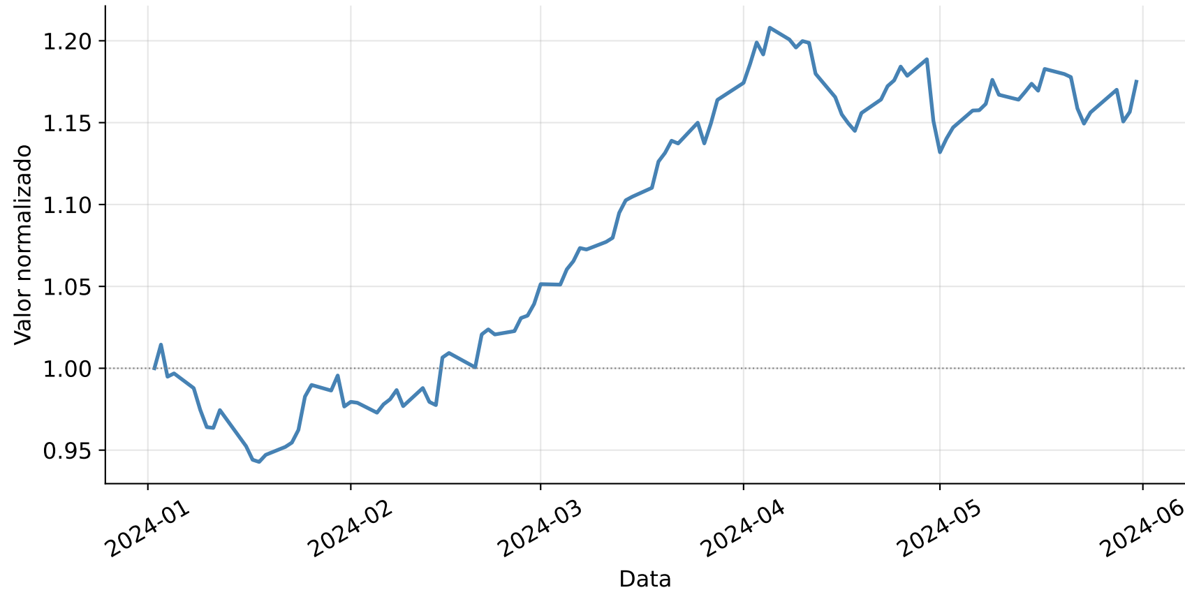
ENERGY — Performance OOS (normalizado)
