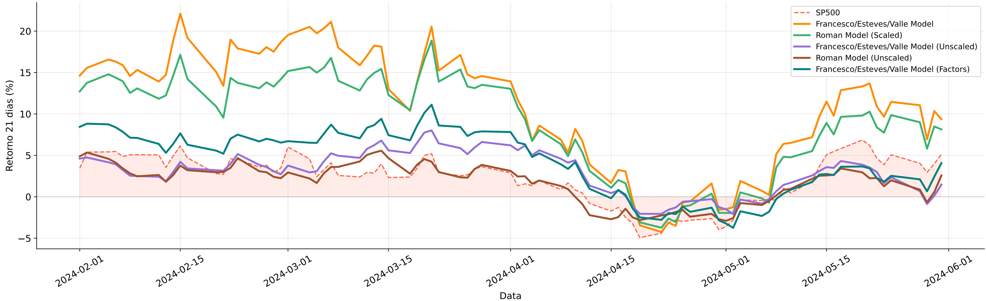
21d return — Francesco/Esteves/Valle Model vs comparisons vs SP500
