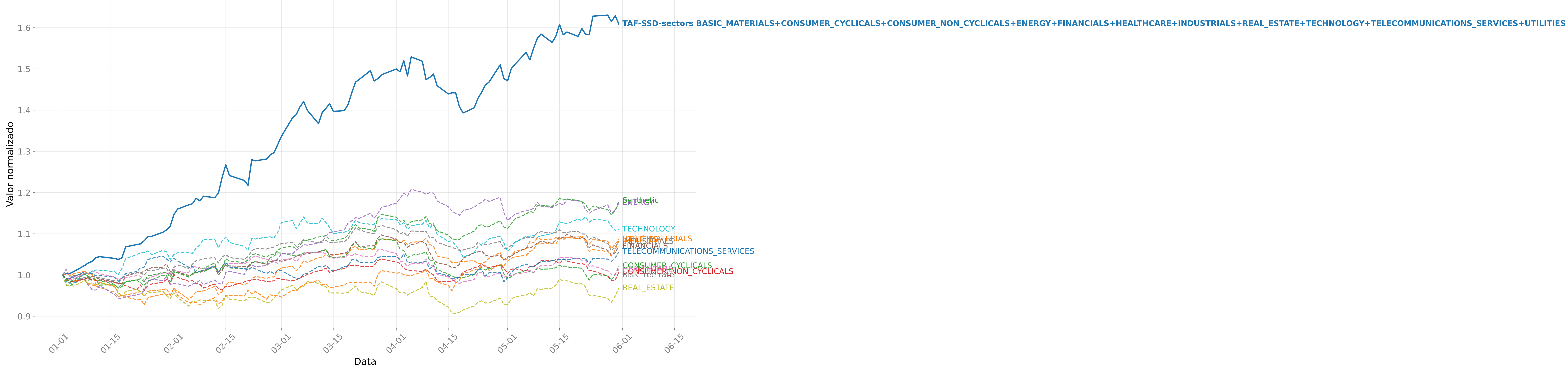
tafmSSD-sectors — TAF-SSD-sectors BASIC_MATERIALS+CONSUMER_CYCLICALS+CONSUMER_NON_CYCLICALS+ENERGY+FINANCIALS+HEALTHCARE+INDUSTRIALS+REAL_ESTATE+TECHNOLOGY+TELECOMMUNICATIONS_SERVICES+UTILITIES vs benchmarks setoriais + sintético (2024-01-01 → 2024-06-01)
