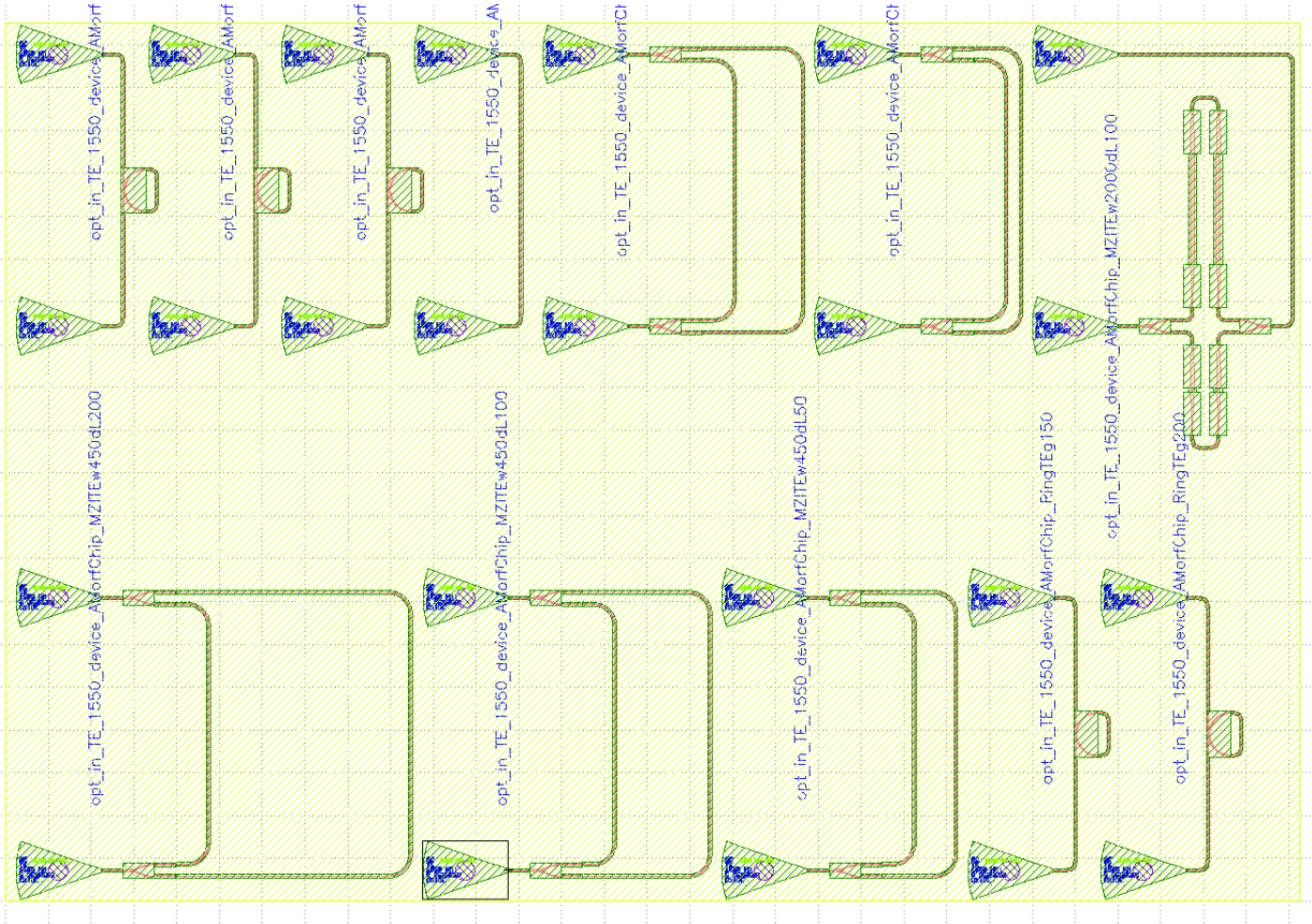
Fig. 6. Layout of EBeam_A_MorfChip ( 605 \times 410 \mu\text{m} ).
