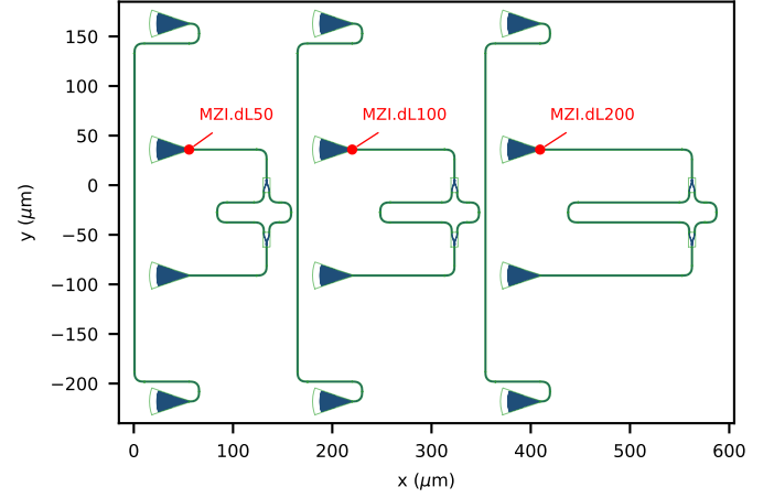
Fig. 5. Layout of the three MZIs ( \Delta L = 50, 100 and 200 \mu\text{m} , from left to right). Blue: silicon (layer 1/0); green outlines: device boundaries; red dots: measurement labels, placed on the second grating coupler from the top of each fibre array. The outer two grating couplers of each array are connected by a loopback waveguide.
