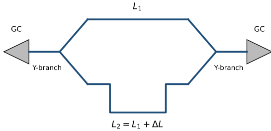
Fig. 2. Schematic of the unbalanced MZI (not to scale): input and output grating couplers (GC), two Y-branches, a short arm of length L_1 and a long arm of length L_2 = L_1 + \Delta L .
