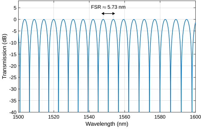
Fig. 4. Transmission of the MZI with \Delta L = 100 \mu\text{m} , computed from the compact model with ideal 50:50 splitters and no loss. Values below -40 \text{ dB} are cut off.
