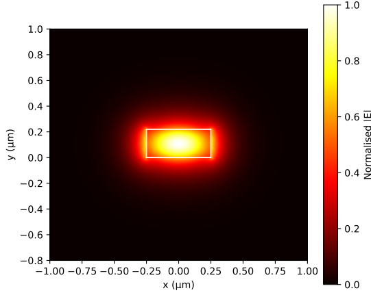
Fig. 1. Normalised |E| of the fundamental quasi-TE mode of the 500 \text{ nm} \times 220 \text{ nm} strip waveguide at 1550 \text{ nm} (Lumerical MODE FDE). The white rectangle is the silicon core.
