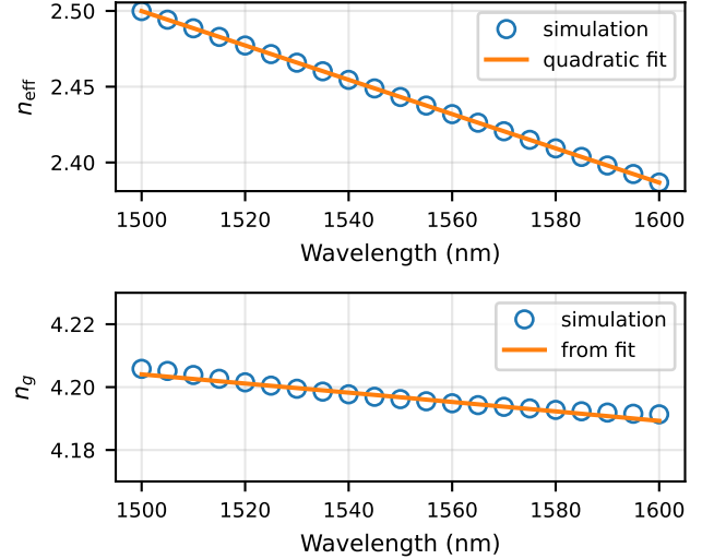
Fig. 3. Effective index (top) and group index (bottom) of the quasi-TE mode versus wavelength. Markers: simulation. Lines: second-order compact model, and the group index computed from it.
