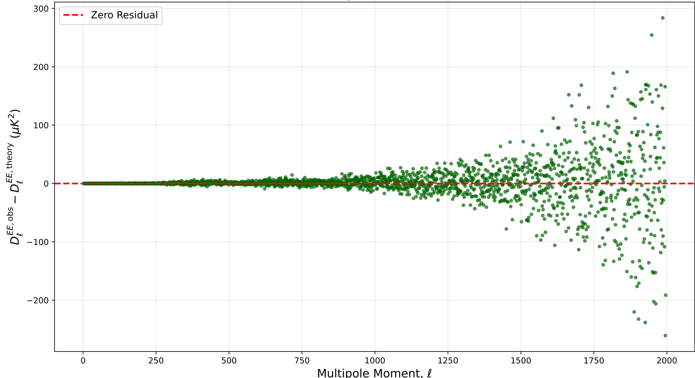
Residuals of the Planck 2018 EE Power Spectrum Relative to the CAMB \Lambda CDM Prediction
