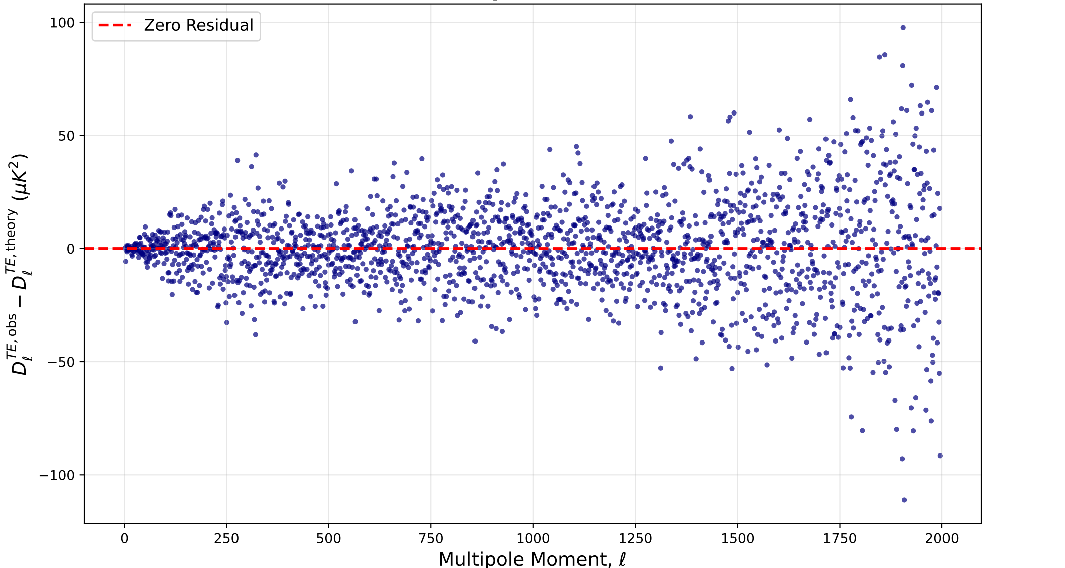
Residuals of the Planck 2018 TE Power Spectrum Relative to the CAMB \Lambda CDM Prediction
