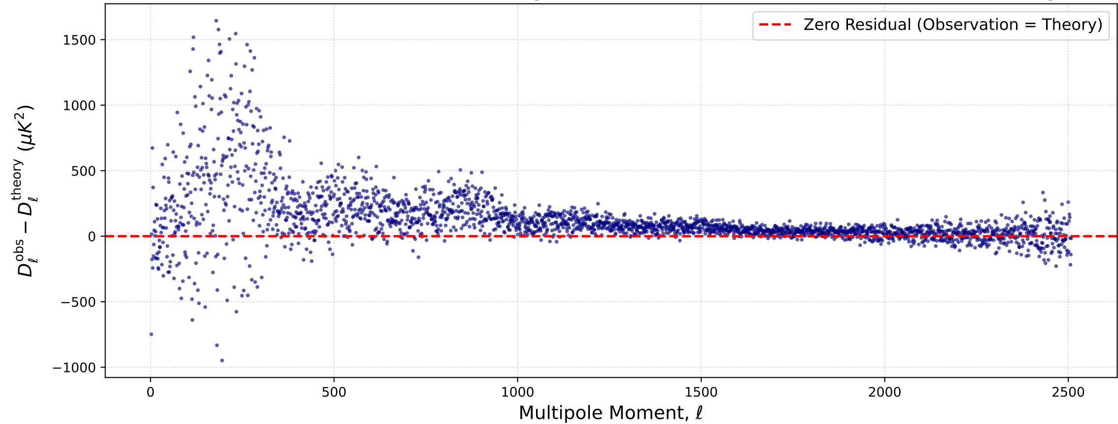
Residuals between the Planck 2018 TT Power Spectrum and the Best-Fit \Lambda CDM Model Computed with CAMB
