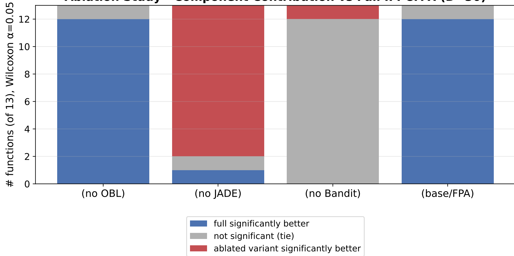
Ablation Study - Component Contribution vs Full IFPOA-X (D=30)
