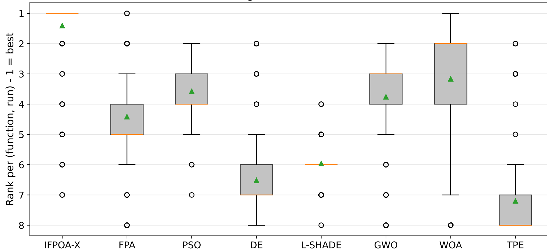
Rank Distribution Across Algorithms (D=50, 13 functions x 20 runs)
