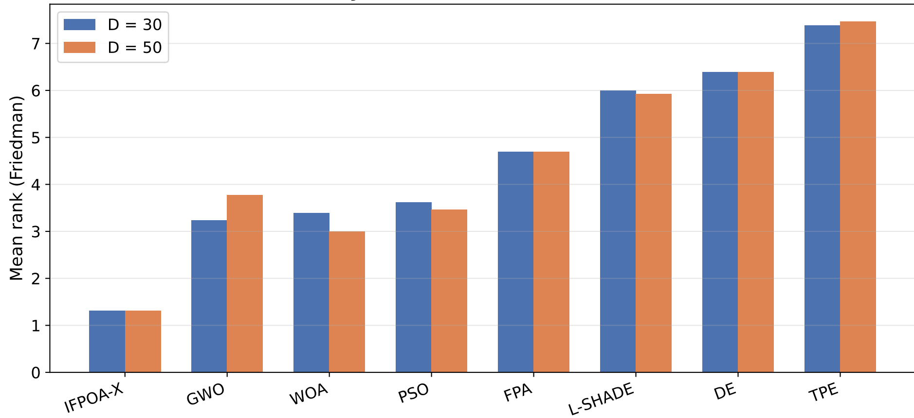
Rank Stability Across Dimensions (D=30 vs D=50)
