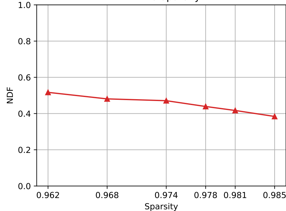
NDF vs Sparsity
