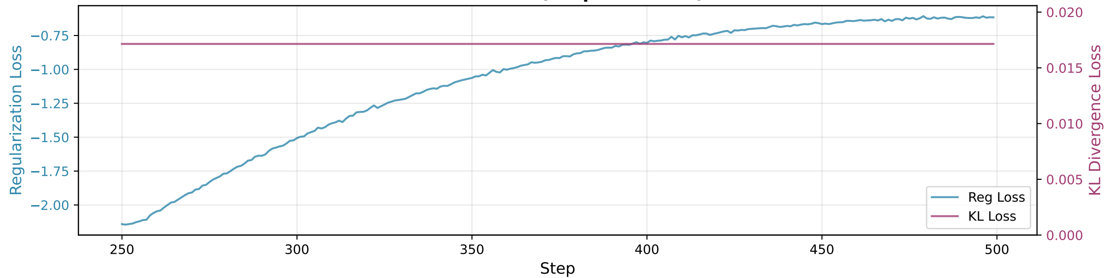
Both Losses (Steps 250-500)
