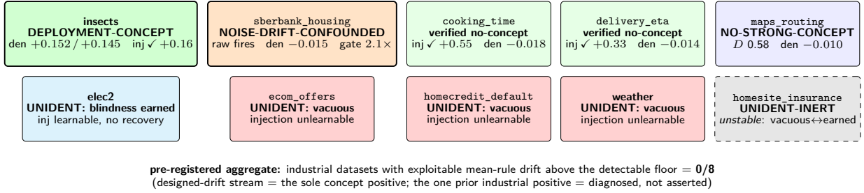
Figure 2: The identifiability map at a glance (Table 4 is the precise record). Tile color encodes the verdict class: green = rule-change verdict or verified no-concept; amber = diagnosed noise mechanism; blue = identifiable null; light blue = earned blindness; red = certificate refused; grey (dashed) = unstable across seed sets. Each tile carries its load-bearing number (denoised staleness, exploratory/confirmatory where both exist, or injection recovery). Color is redundant: every tile also prints its verdict.
