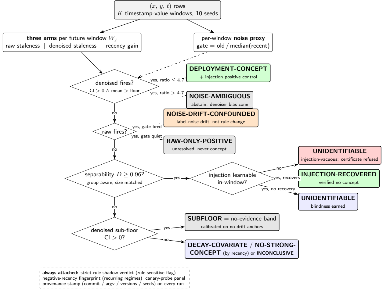
Figure 1: The decision cascade of the instrument. The cascade is specified verbatim in §3.3 and PREREG §3. Side channels attached to every run: the strict-rule shadow verdict (rule-sensitive flag), the negative-recency fingerprint for recurring regimes (§6), the canary-probe panel (§4.3), and provenance stamping on every run.
