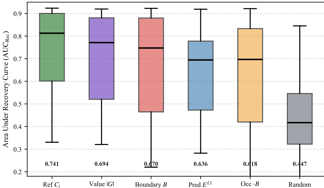
Empirical Distribution of Recovery AUC across 50 Evaluation Seeds
