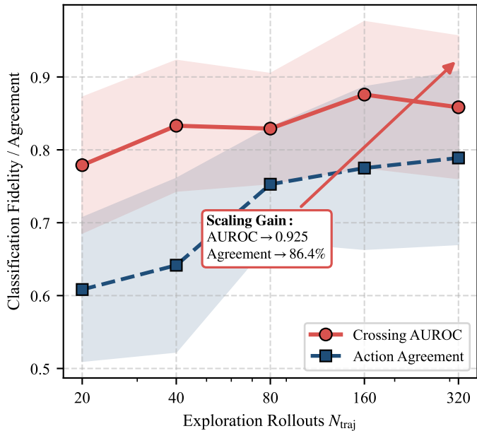
(a) Discriminative Scaling
