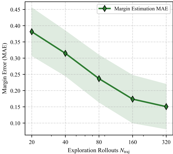
(b) Margin Metric Calibration Error
