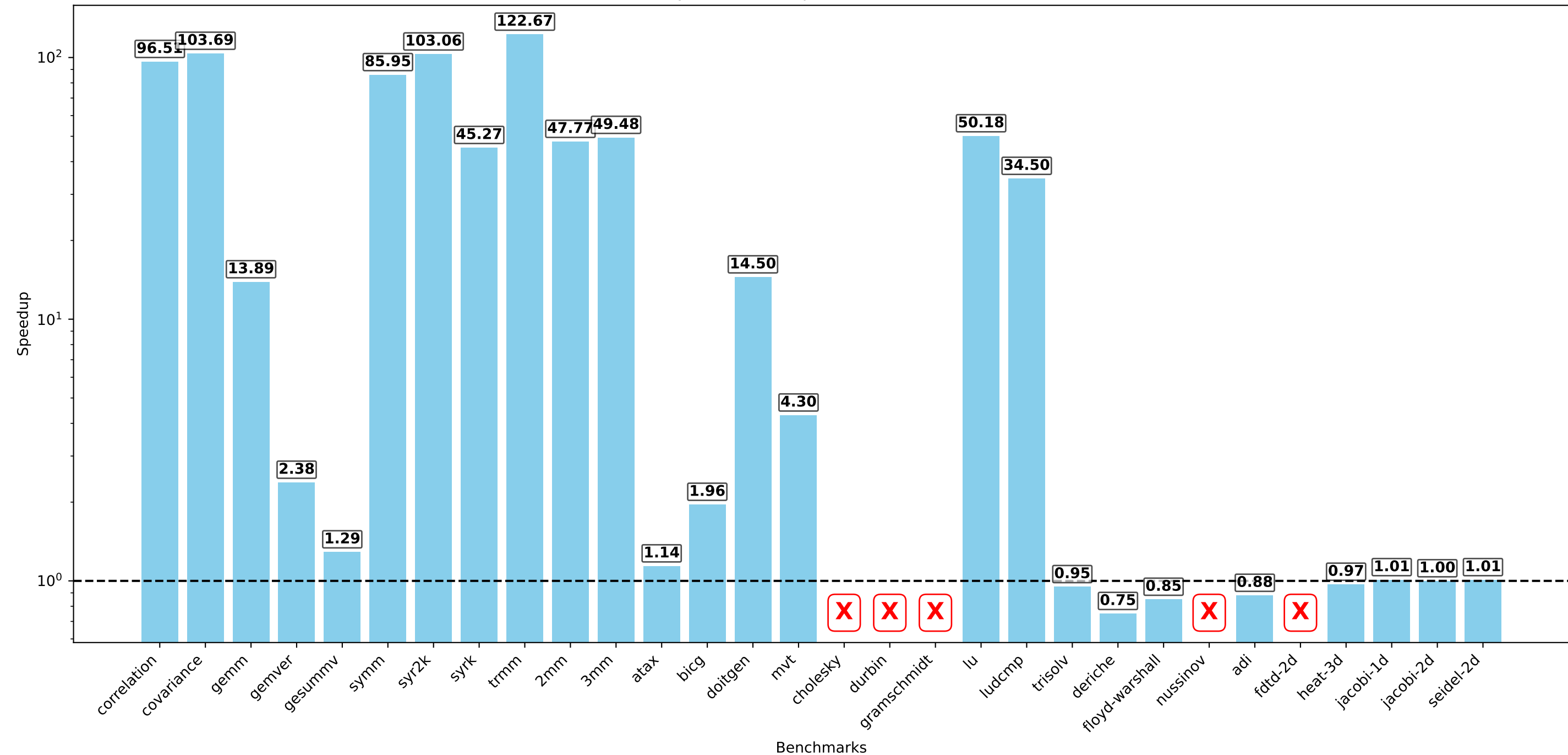
Kernel with MKL library vs. Naive Implementation (X marks indicate failures)
