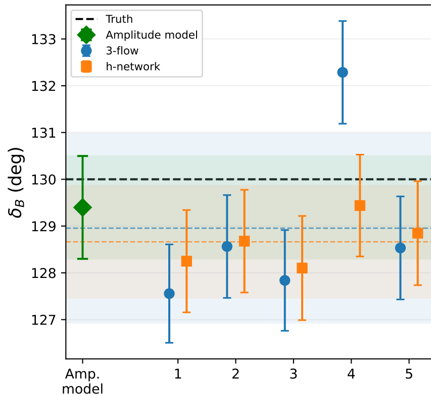
B^\pm \rightarrow DK^\pm fit comparison: amplitude model vs 3-flow vs h-network (shared pseudo-data, r_B=0.1 , 100k B^+ + 100k B^- , 5 datasets)
