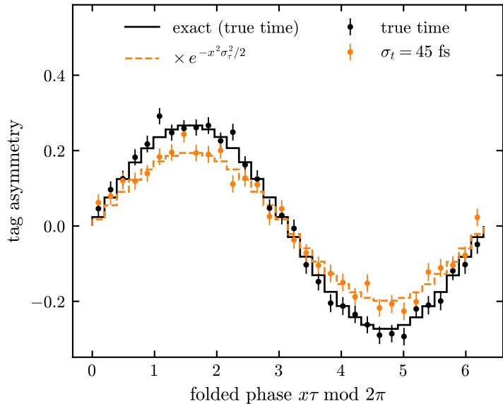
B_s^0, f_0(980) band, test phase \arg(q/p) = -0.4 damping 0.728 \pm 0.016 , expected D = 0.726
