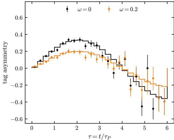
B^0, f_0(980) band: mistag dilutes the asymmetry by 1 - 2\omega
