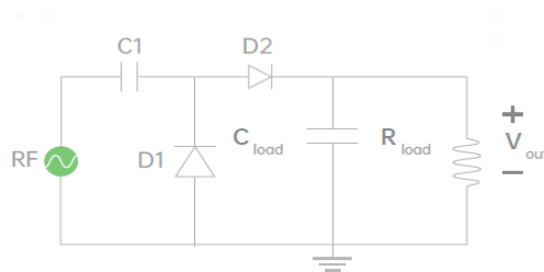
Figure B.1-1: rectifier circuit For RF energy harvesting
