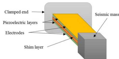
Figure B.1-4: Piezoelectric energy harvesting generator [25]
