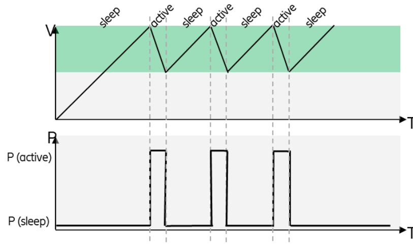
Figure C-2 Example where the active period for the device is relative short
