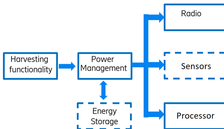
Figure C-1 Example of parts in an Ambient IOT device
