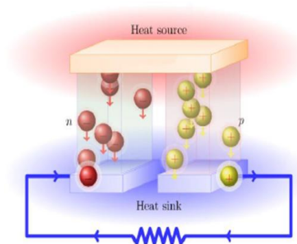
Figure B.1-3: Seebeck effect
