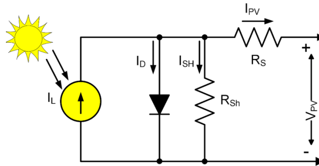
Figure B.1-2: The equivalent electrical circuit of a single diode solar PV cell [21]
