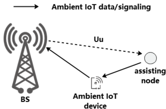
Figure 4.2.1.3-1: Topology 3 with downlink assistance
