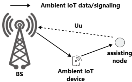
Figure 4.2.1.3-2: Topology 3 with uplink assistance
