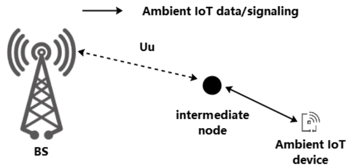
Figure 4.2.1.2-1: Topology 2
