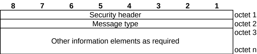
Figure 7.1.1.2-1: General message organization example for an unprotected AIoT NAS message
