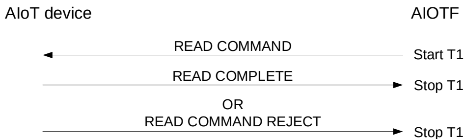
Figure 5.3.2.1-1: Read command procedure
