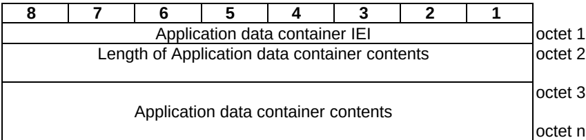
Figure 7.2.14-1: Application data container information element
