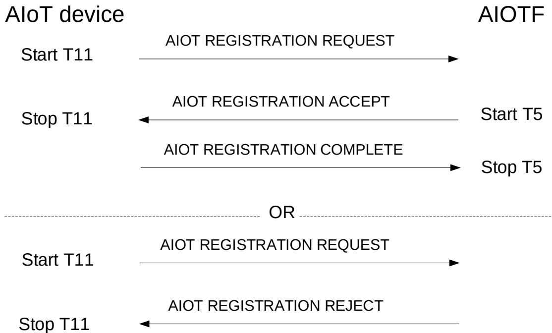
Figure 5.5.2.1-1: AIoT Registration procedure
