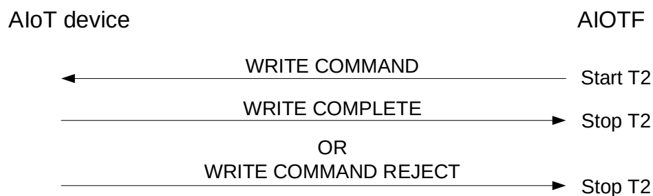
Figure 5.3.3.1-1: Write command procedure
