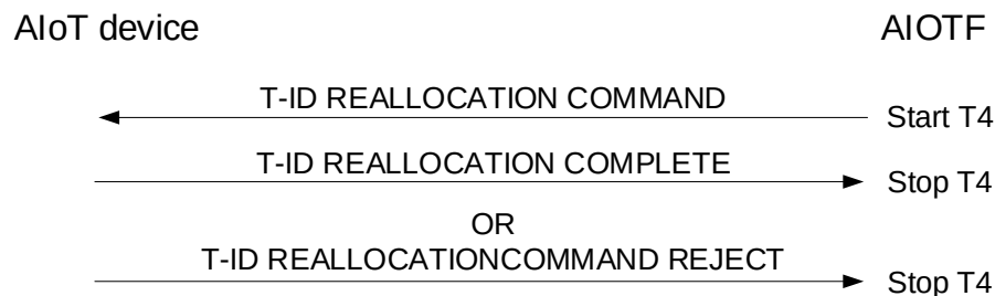
Figure 5.4.2.1.1: T-ID reallocation command procedure
