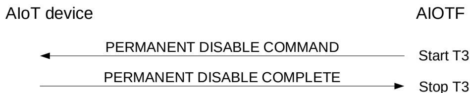
Figure 5.3.4.1-1: Permanent disable command procedure
