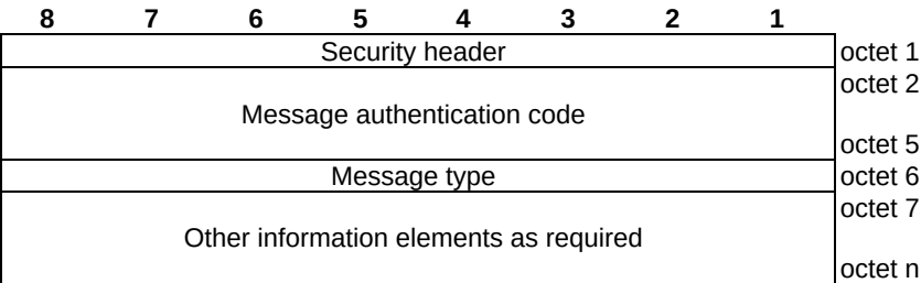
Figure 7.1.1.2-2: General message organization example for a security protected AIoT NAS message
