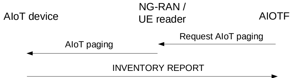
Figure 5.2.2-1: Inventory procedure
