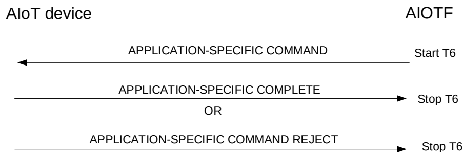
Figure 5.3.5.1-1: Application-specific command procedure
