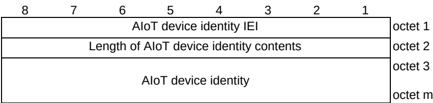
Figure 7.2.6-1: AIoT device identity information element
