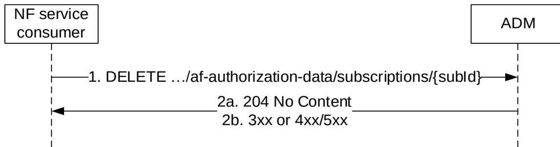
Figure 5.2.2.5.2-1: Delete a subscription of AF Authorization Data change
