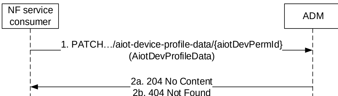
Figure 5.2.2.3.2-1: Updating AIoT Device Profile Data
