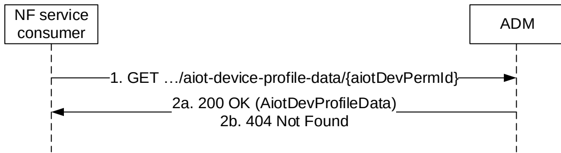
Figure 5.2.2.2-1: Requesting AIoT Device Profile Data
