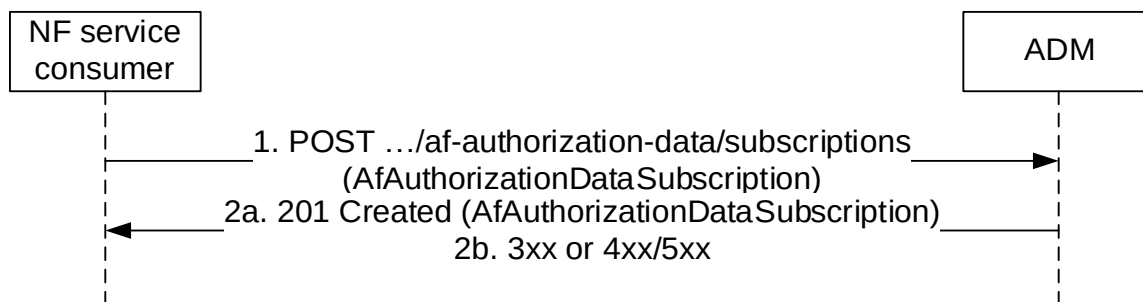
Figure 5.2.2.4.2-1: Create a subscription of AF Authorization Data change
