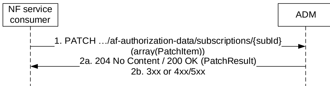
Figure 5.2.2.4.3-1: Modify a subscription of AF Authorization Data change
