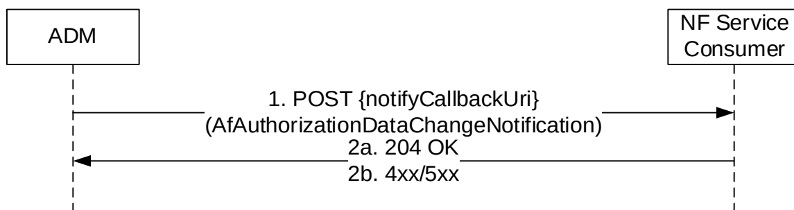
Figure 5.2.2.6.2-1: Notify changes of AF Authorization Data
