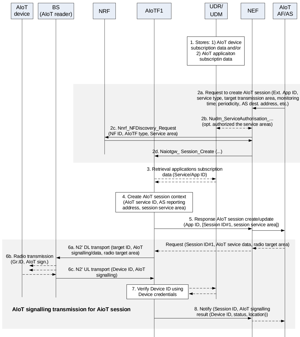
Figure 6.19.3.2-1: Signalling flow for AIoT session establishment between the AIoTF and the AIoT AF/AS and AIoTF and the BS AIoT Reader via the N2' association for a particular target area
