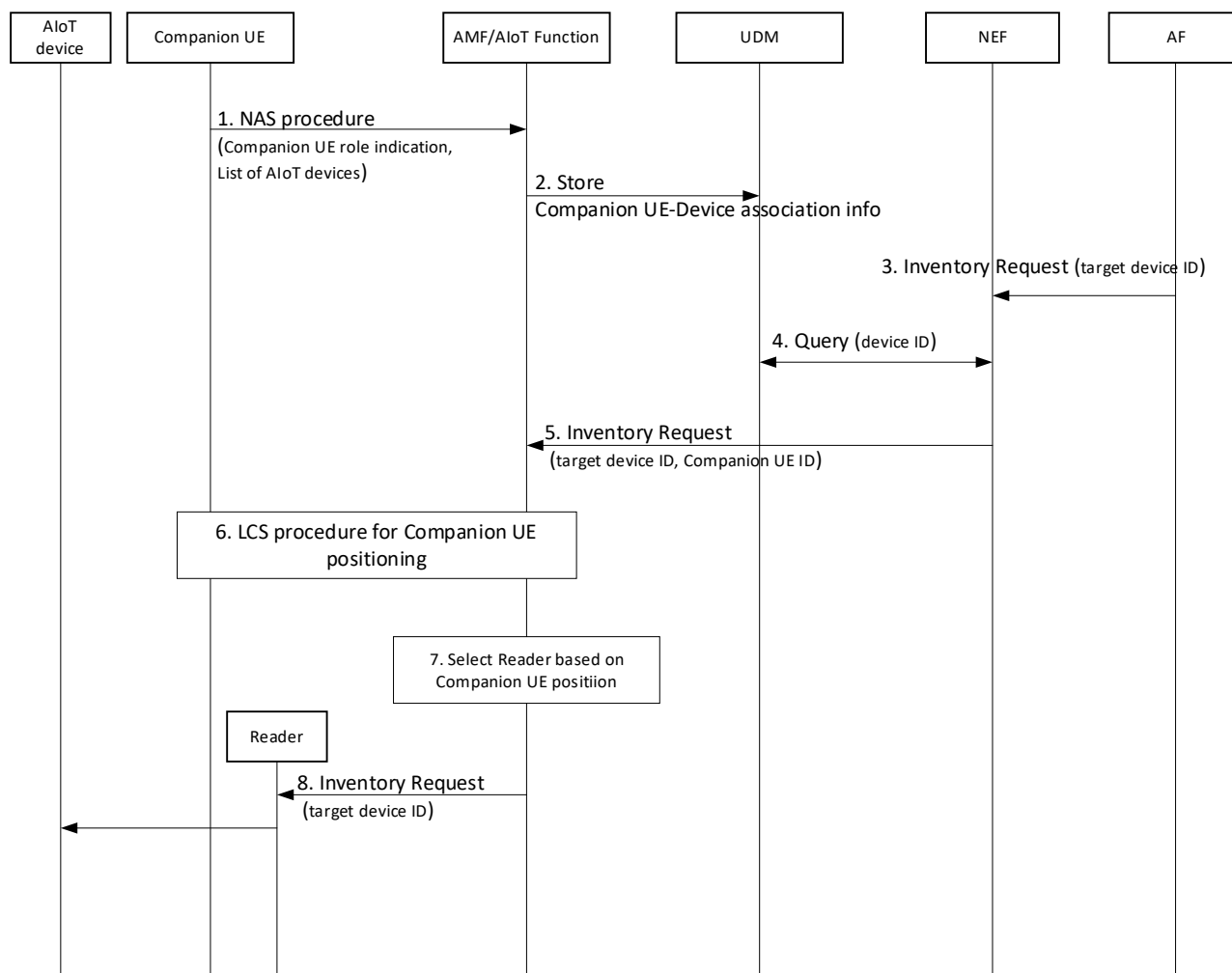
Figure 6.38.2-1: AIoT inventory procedure using Companion UE
