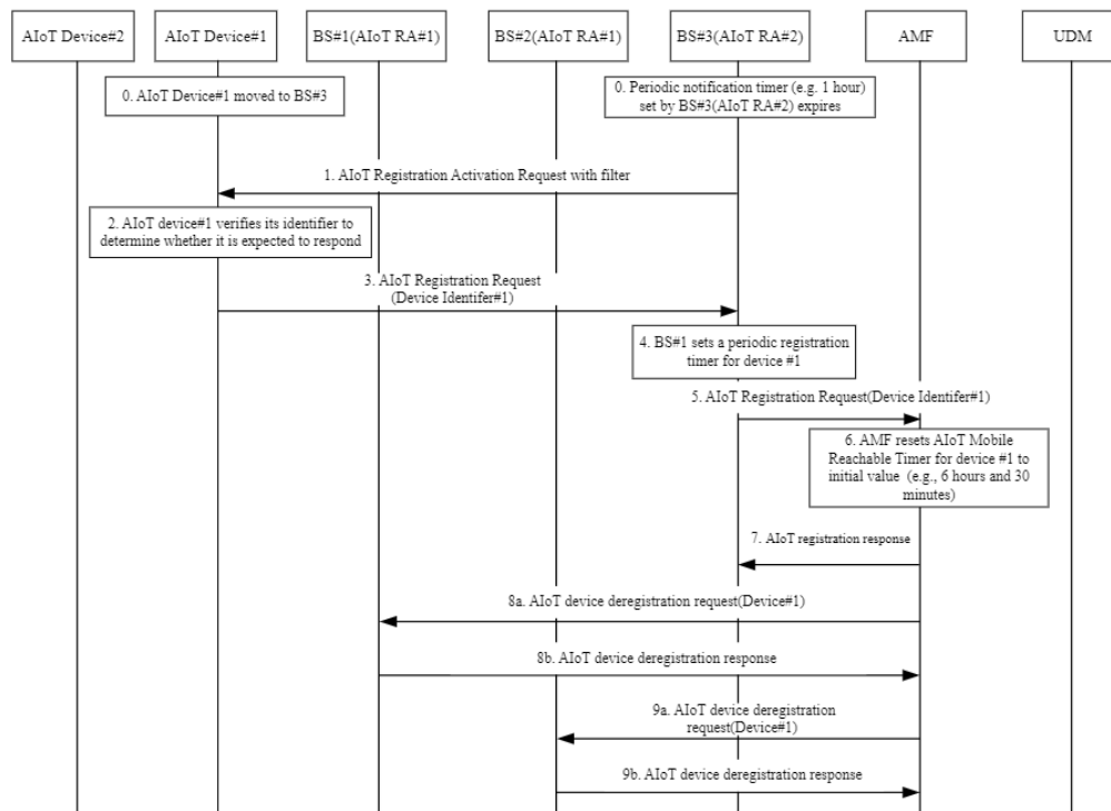
Figure 6.29.2.3-1: BS relocation according the update of the latest registration area of AIoT device
