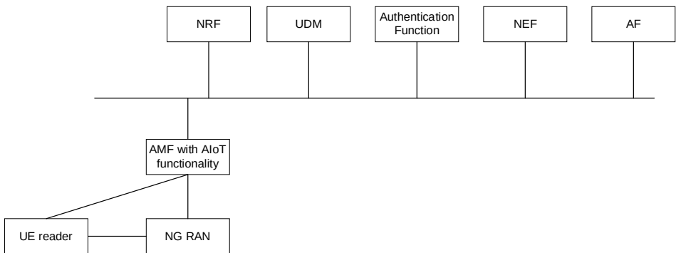
Figure 6.4.1.4.1-3: The example of reference architecture for alternative 2
