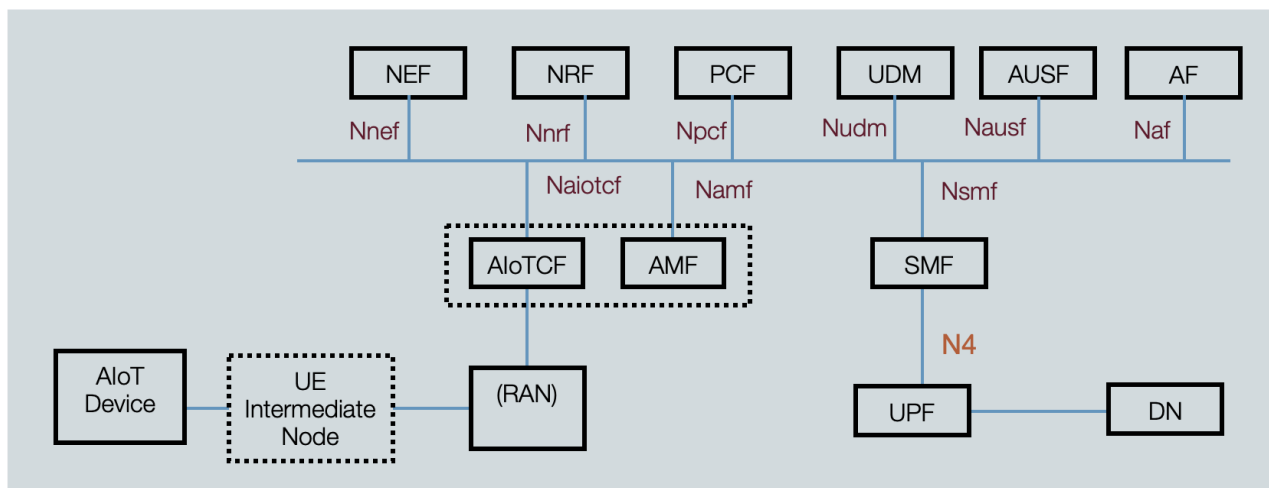
Figure 6.33.1.3-1: Reference Architecture to support Ambient IoT
