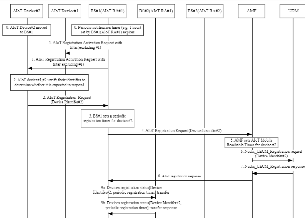
Figure 6.29.2.2-1: Periodic triggered AIoT devices to perform Registration Update (Continued)
