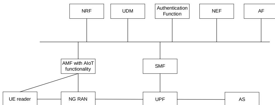
Figure 6.4.1.4.2-1 An example of reference architecture for discovering UE reader via control plane and AIoT device related data delivery via UE reader user plane
