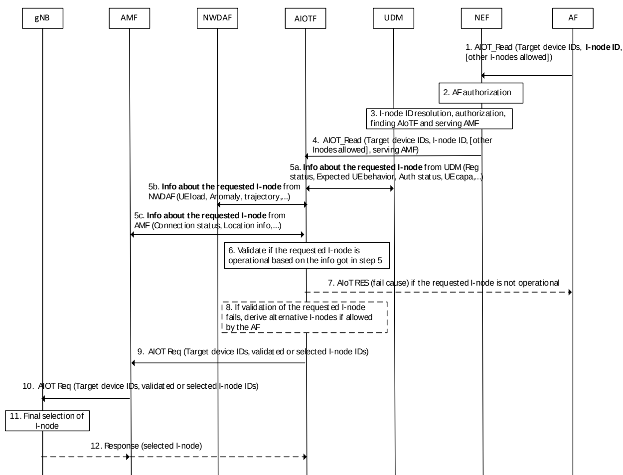
Figure 6.11.2.2-3: Information Flow for selection of I-nodes based on list of I-nodes from AF
