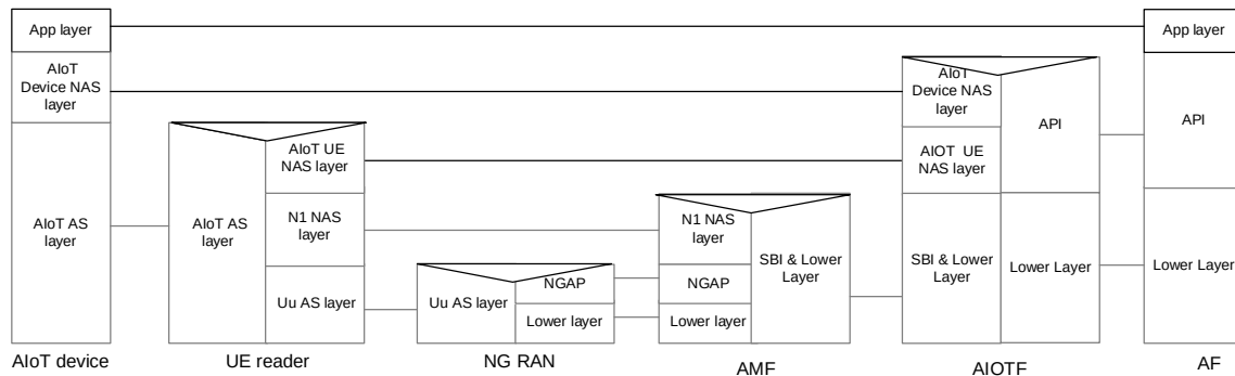
Figure 6.30.1.2-1: Protocol Stack for Supporting AIoT Devices using AIOTF for Topology 2
