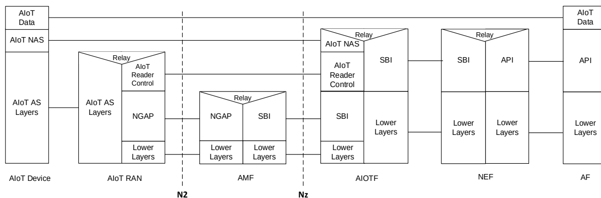
Figure 8.1.2.3-3: Example Protocol Between AIOTF and AIoT Device for Topology 1 (indirect Path via AMF)
