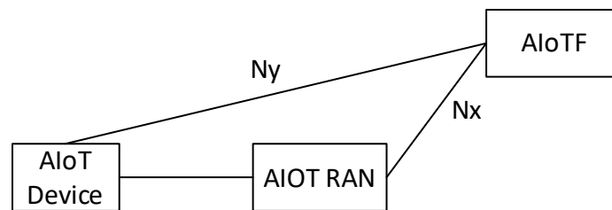
Figure 8.1.2.2-2: Non-Roaming 5G System Architecture in reference point representation (Direct Path)
