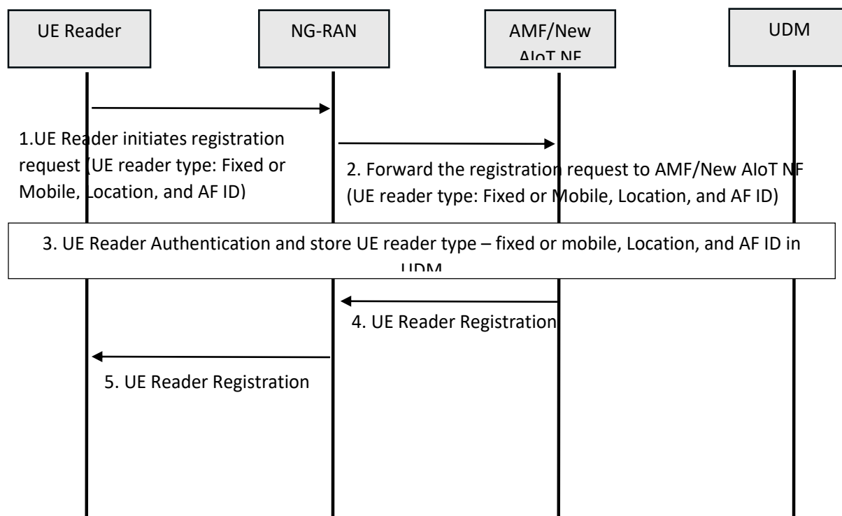
Figure 6.31.2.1-1: Reader UE registration procedure with UE reader type info, location, and AF ID
