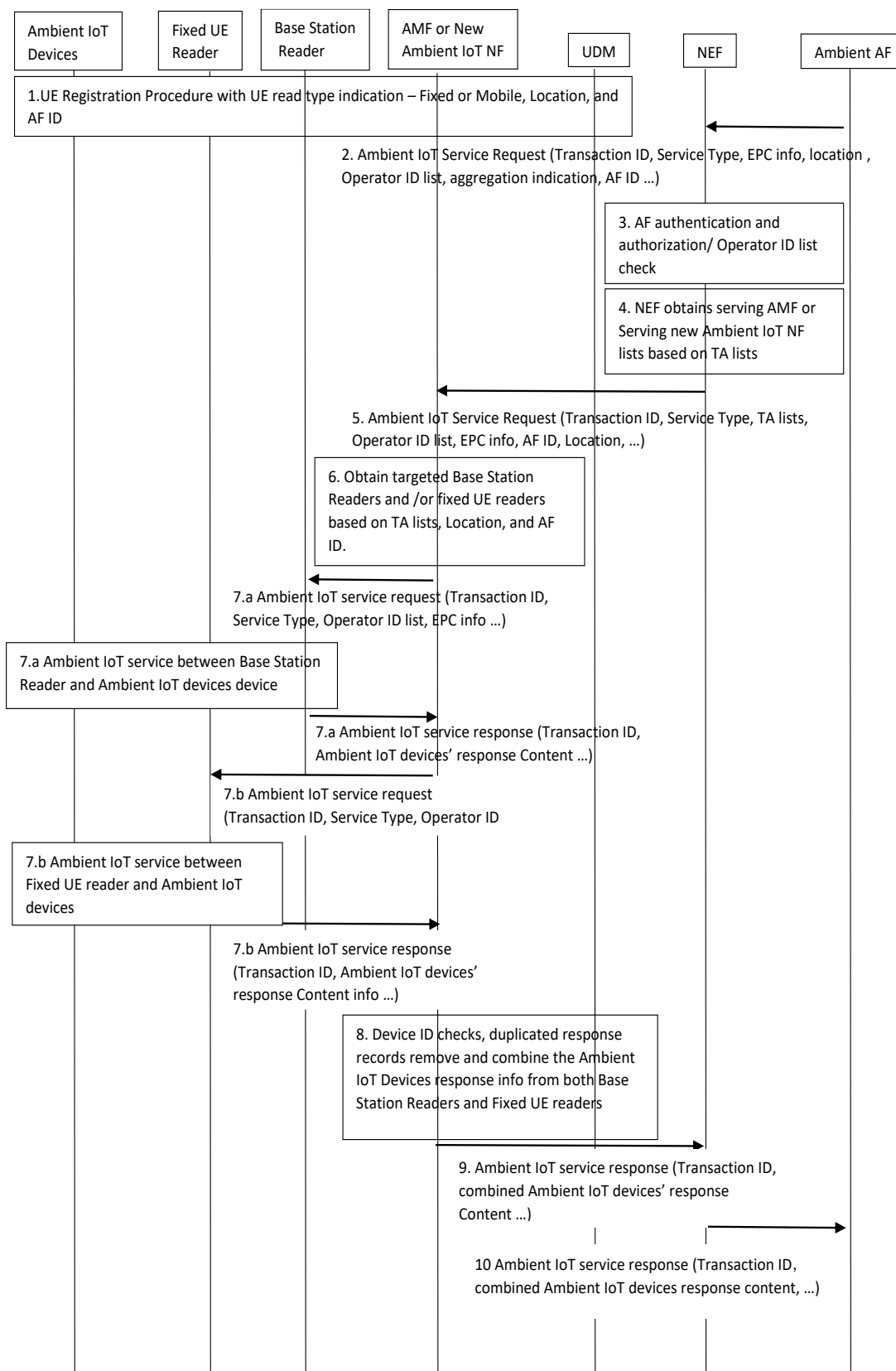
Figure 6.31.2.2-1: Network initiated ambient IoT service procedure with fixed UE reader
