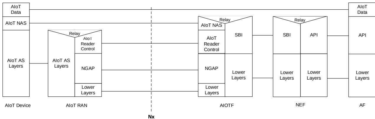
Figure 8.1.2.2-3: Example Protocol Stack between AIOTF and AIoT Device for Topology 1 (Direct Path)
