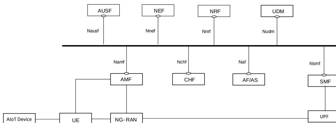
Figure 6.22.1.1-1: System Architecture of AF Based Solution
