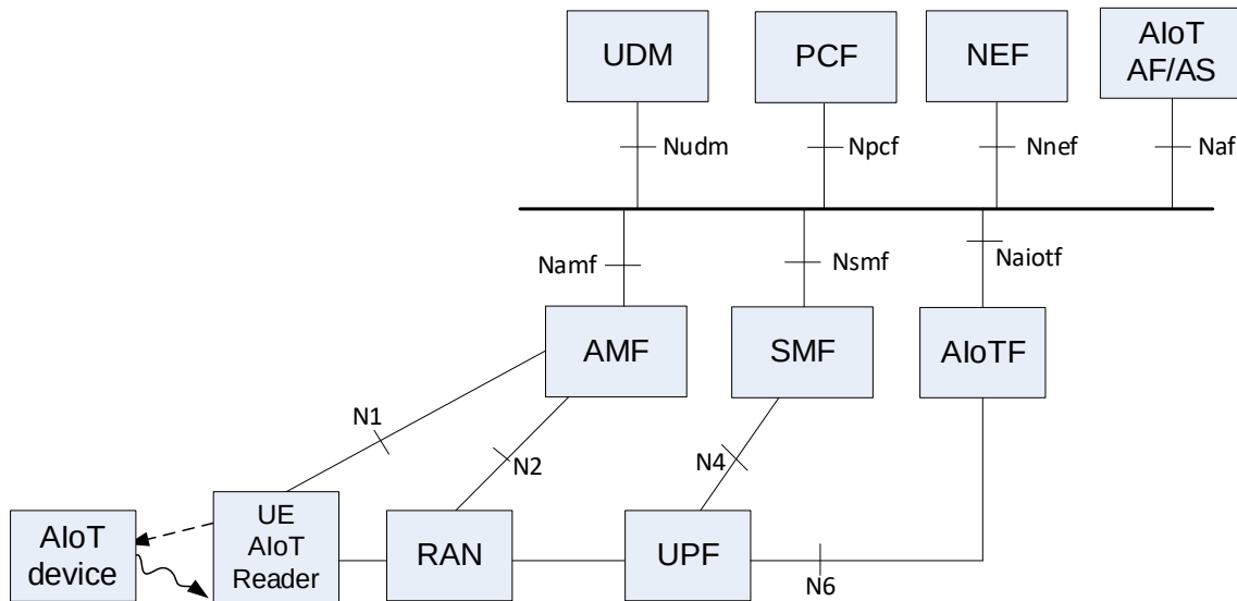
Figure 6.32.2.1-1: Assumed architecture for AIoT services using topology 2 and AIoT data transmission in the UP of a PDU Session
