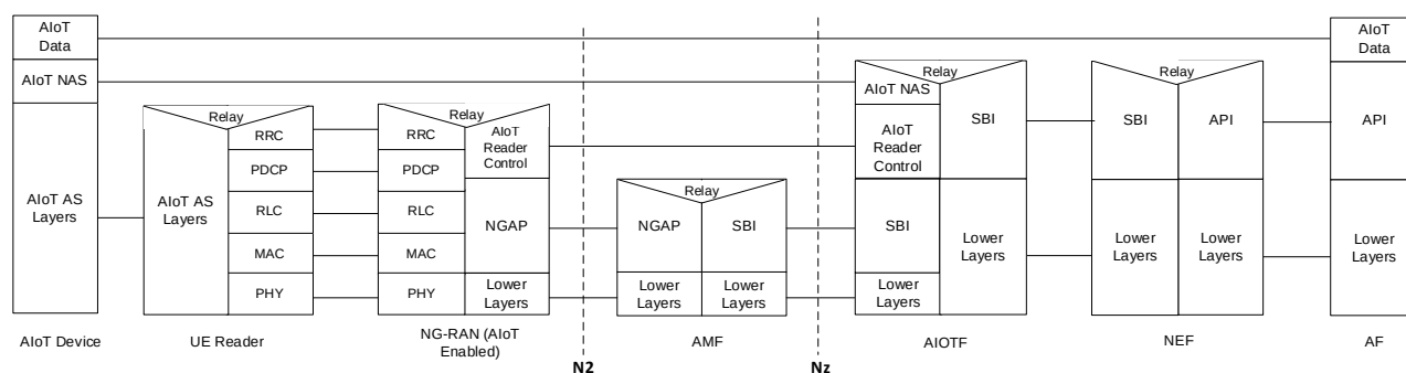
Figure 8.1.3.3-1: Protocol Stack for the RRC option
