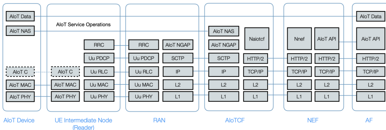
Figure 6.33.1.4-1: Protocol Stack to support Ambient IoT
