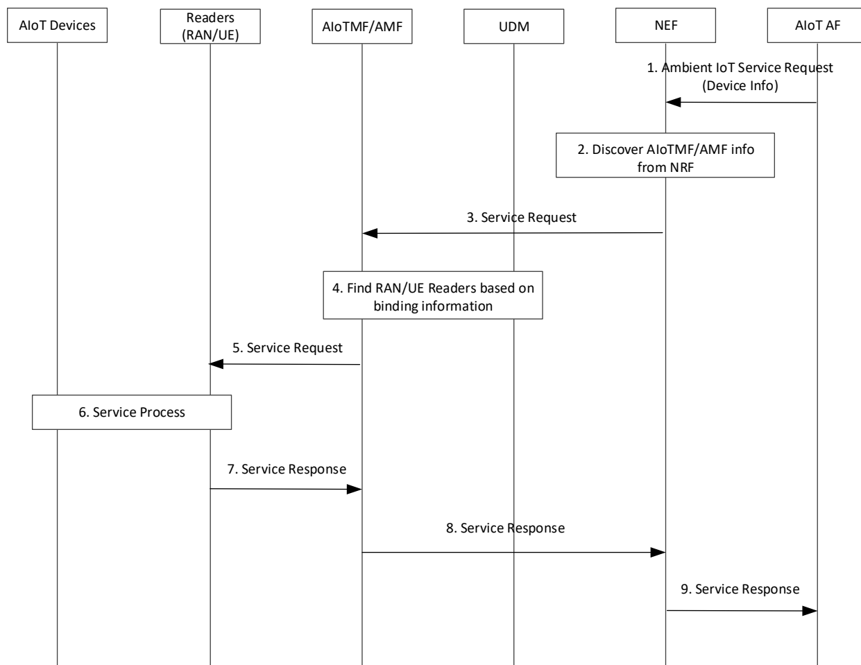
Figure 6.28.2.2-1: Device-Reader binding information usage
