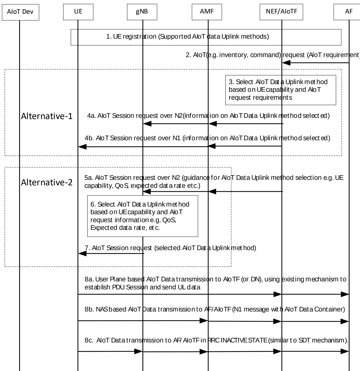
Figure 6.42.2-1: Information Flow for AIoT communication optimization
