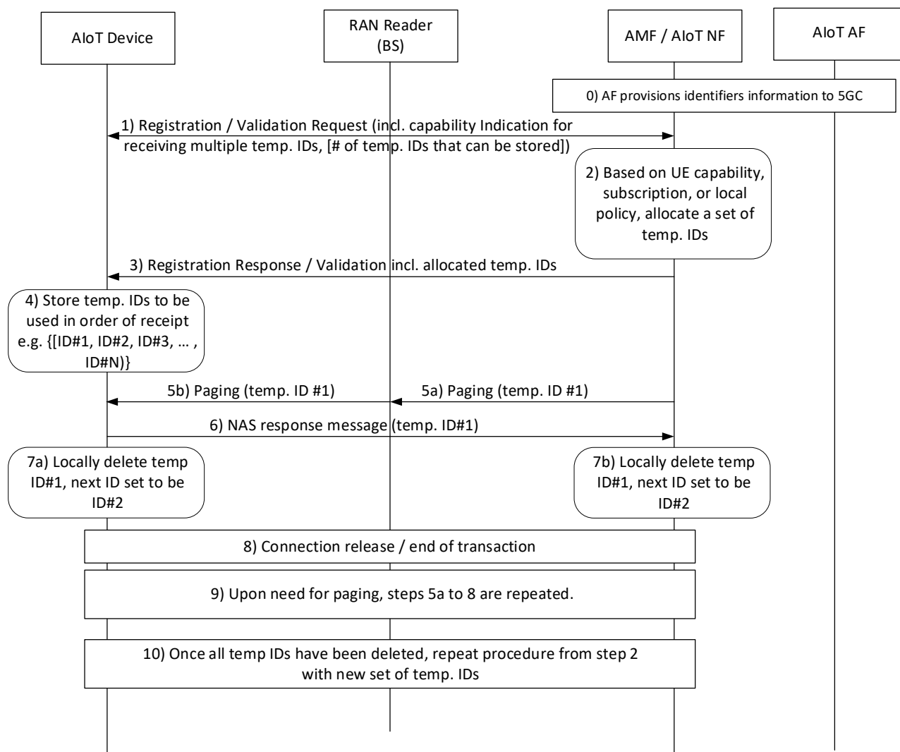
Figure 6.37.2.1-1: Procedure to support allocation of multiple temporary identities to AIoT devices
