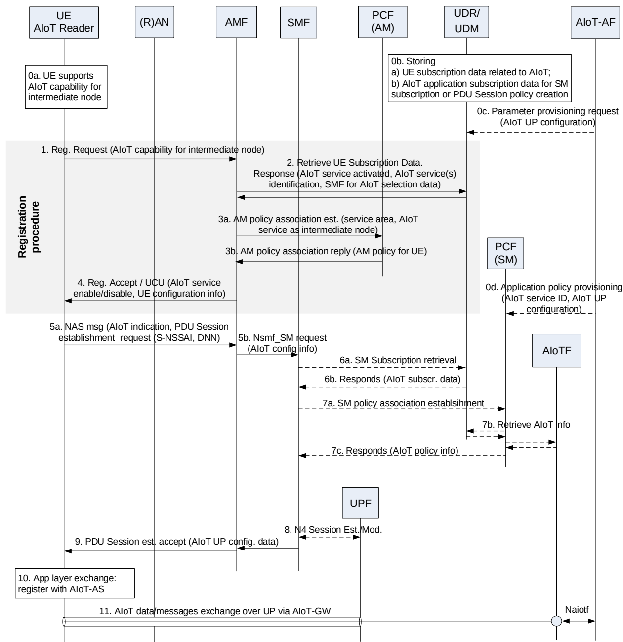
Figure 6.32.3-1: Signalling flow of the AIoT session establishment between the UE AIoT Reader and the AIoTF or AIoT-AS in the U-plane
