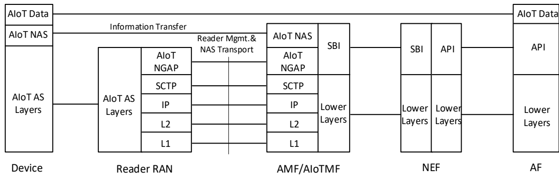
Figure 6.17.1.3-1: AIoT Protocol Stack (Topology 1)
