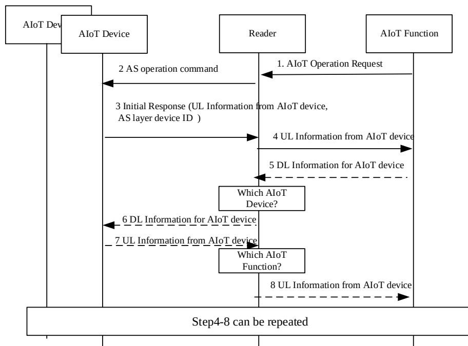
Figure 6.20.1-1: interaction for AIoT Device related information
