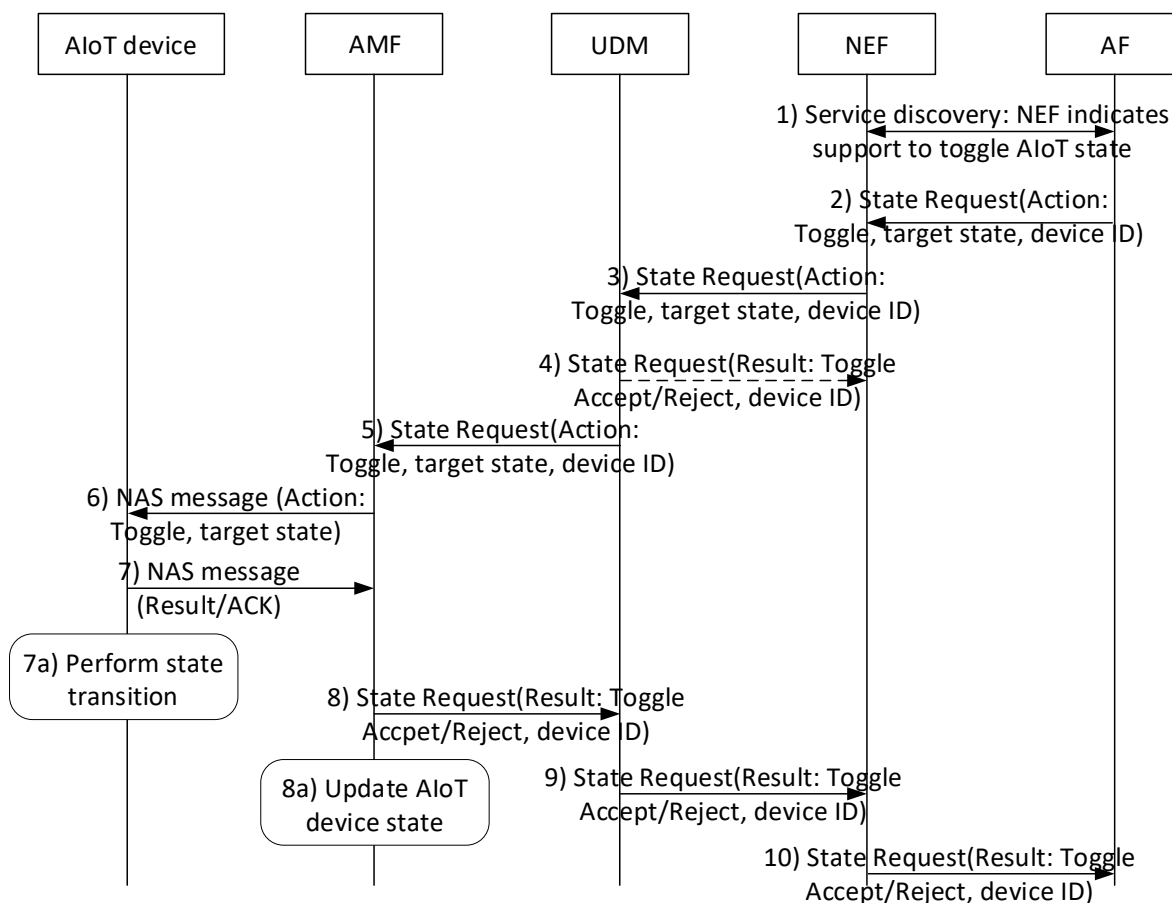
Figure 6.15.2-1: Procedure to support toggling of states in an AIoT device
