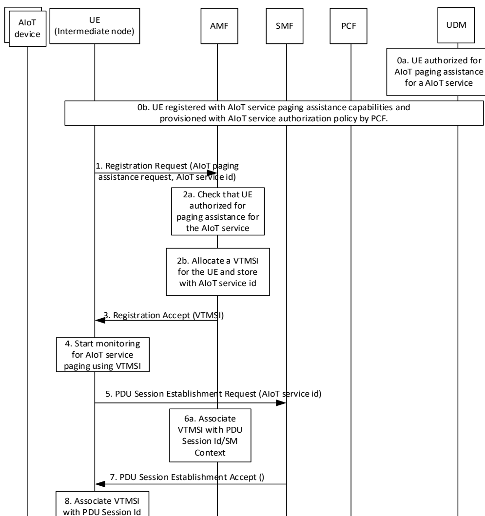
Figure 6.34.2-1: UE Registration and PDU Session establishment procedures
