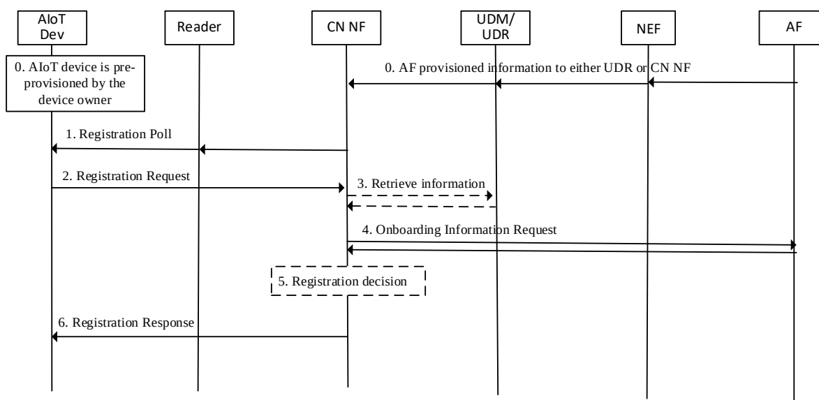
Figure 6.16.2-1: Registration/onboarding procedure for an AIoT device.
