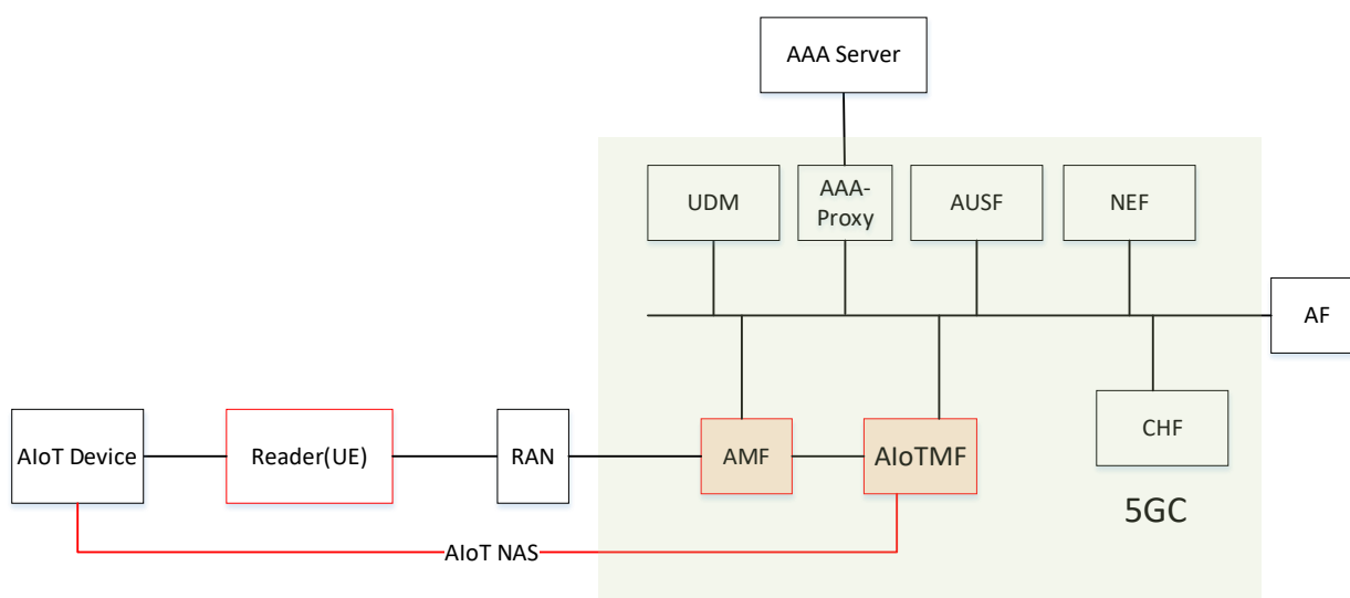
Figure 6.17.1.2-2: 5GC enhancements to support Ambient IoT for topology 2
