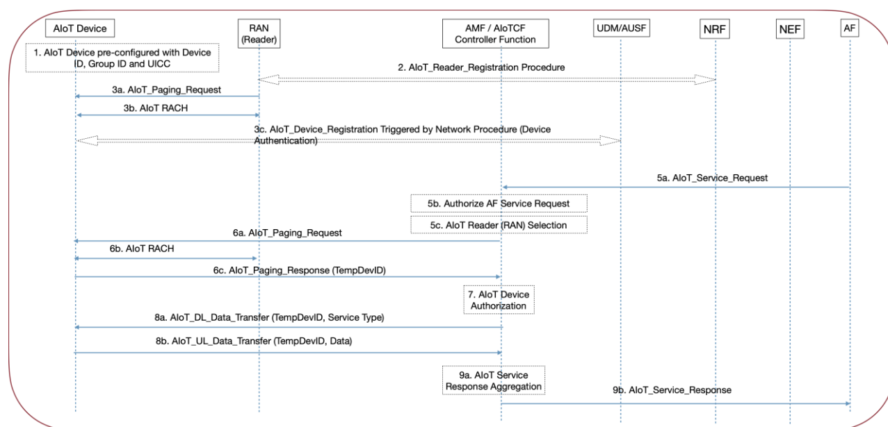
Figure 6.33.2.2-1: AIoT Service Operation Procedure for Type B AIoT Device
