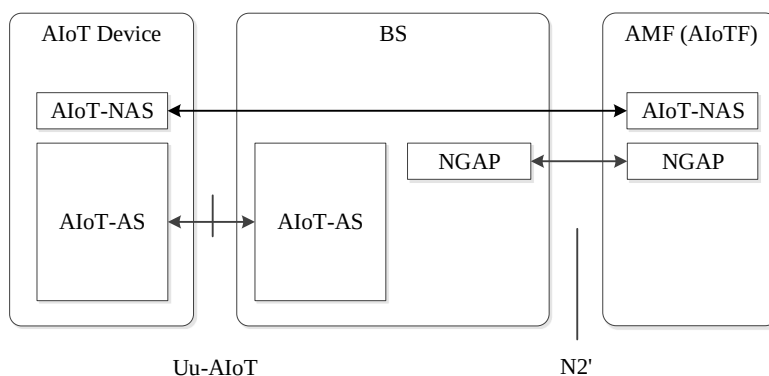
Figure 6.5.1-2: Protocol stack to support AIoT Services for Topology 1
