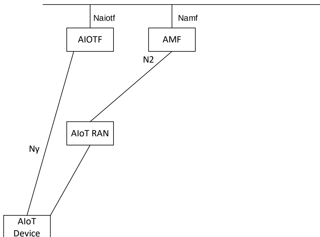
Figure 8.1.2.3-1: Non-Roaming 5G System Architecture (indirect Path via AMF)
