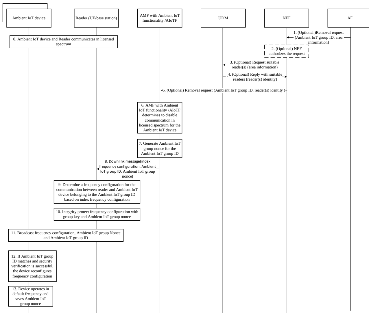
Figure 6.39.2.2-1: Disablement of communication in operator network
