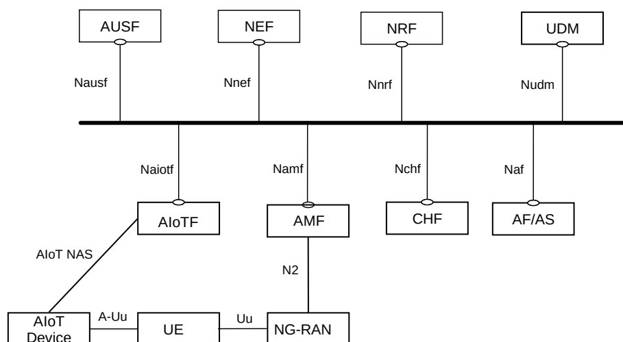
Figure 6.21.1-1: System Architecture to support AIoT Services for Topology 2
