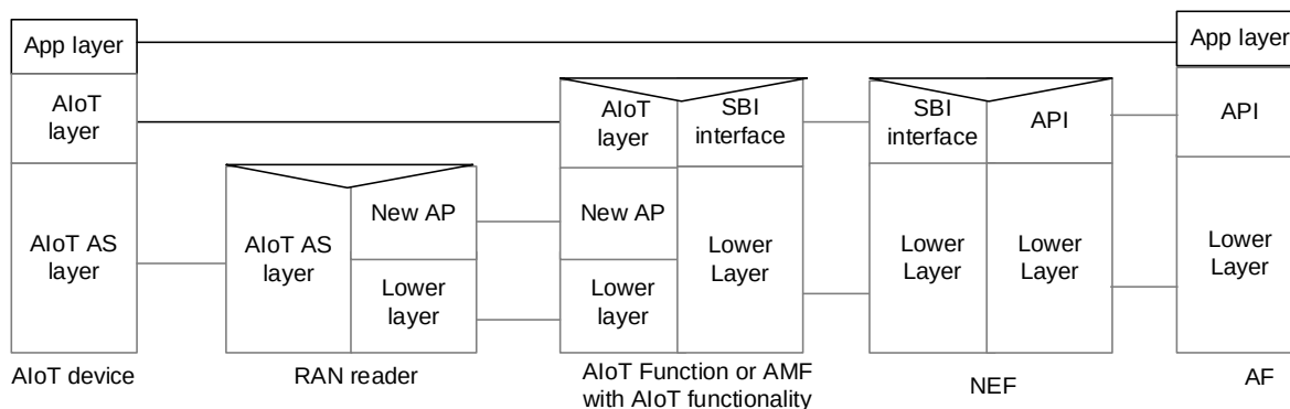
Figure 6.4.1.5-1: protocol stack example for Topology1
