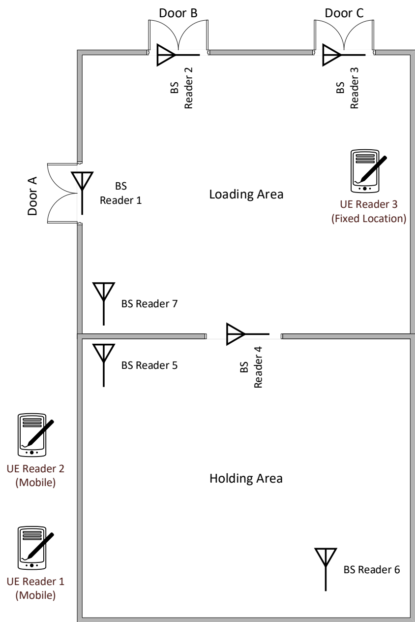
Figure 6.26.1.2-1: Example Target Sets Plan
