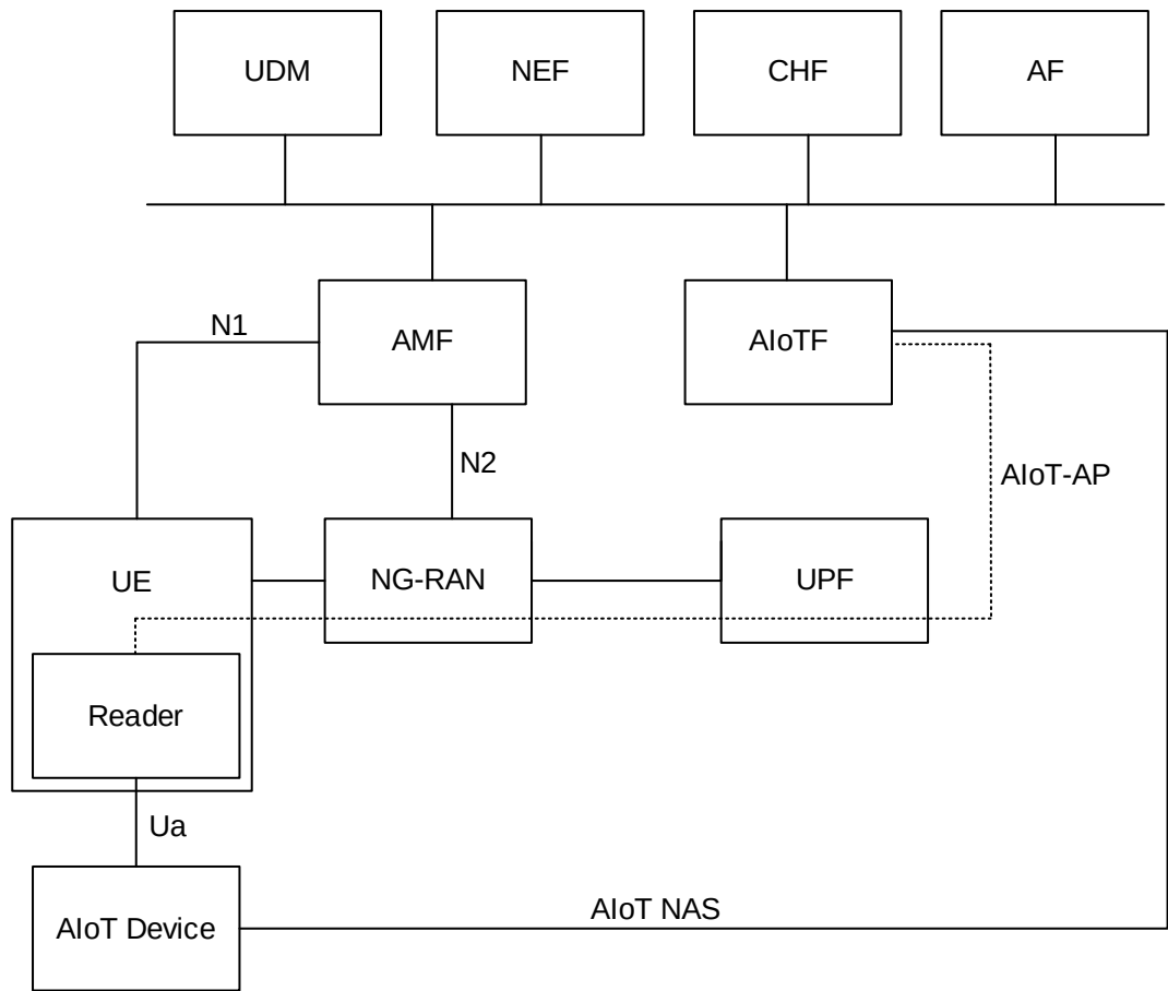
Figure 8.1.3.2-1: User-plane architecture for Topology 2
