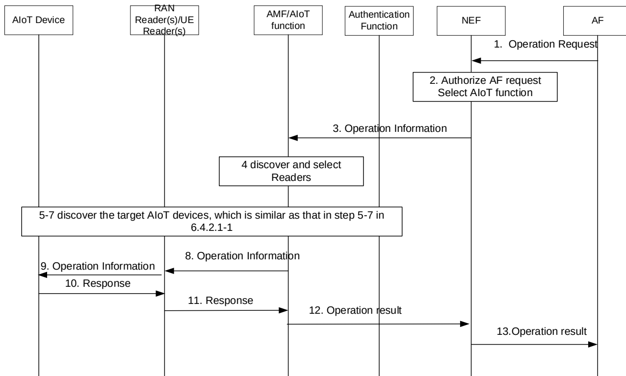
Figure 6.4.2.2-1: Command Service Flow
