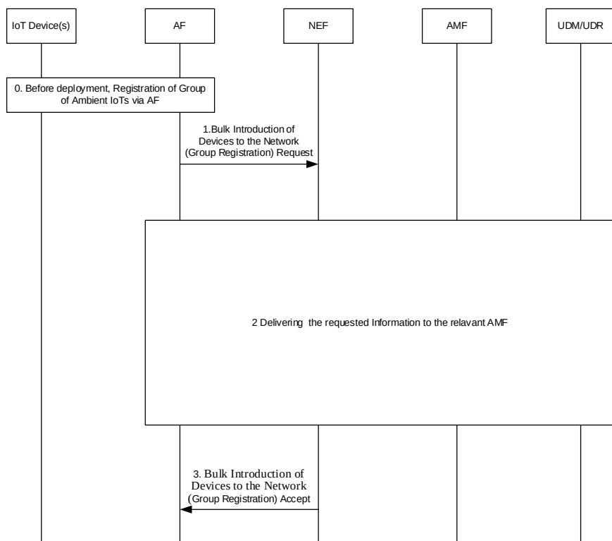
Figure 6.7.2-1: Bulk Introduction of Devices to the Network procedure for Ambient IoT
