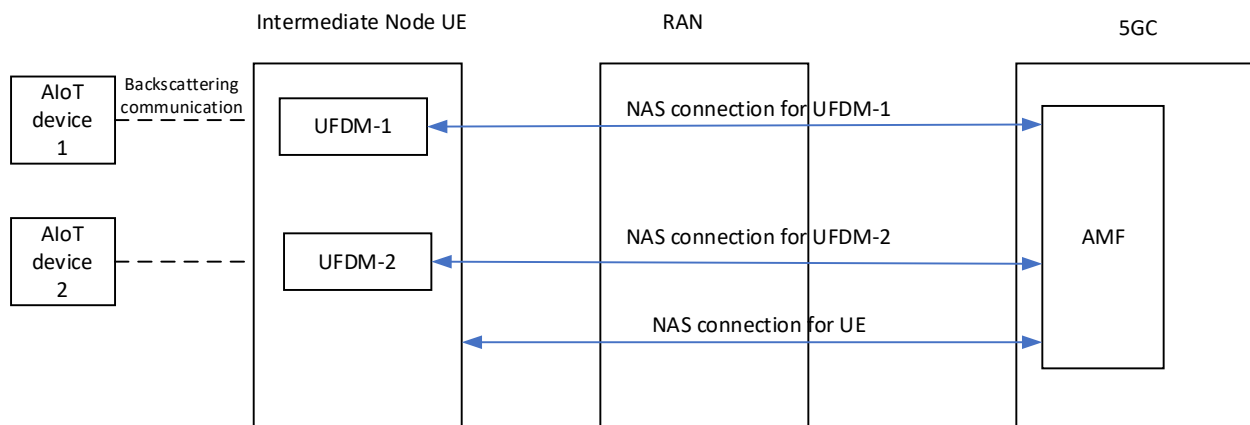
Figure 6.12.1-1: UFDm in AIoT Capable UE for AIoT devices
