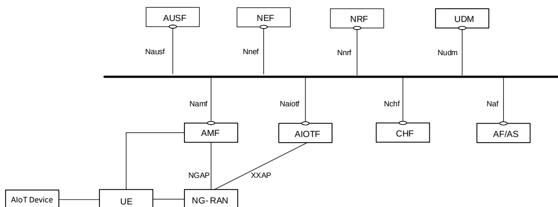
Figure 6.43.1.1-1: System Architecture of harmonized RAN-CN solution using AIOTF for Topology 2
