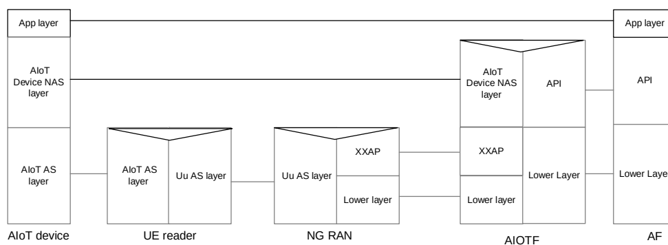
Figure 6.43.1.2-1: Protocol Stack for harmonized RAN-CN solution using AIOTF for Topology 2
