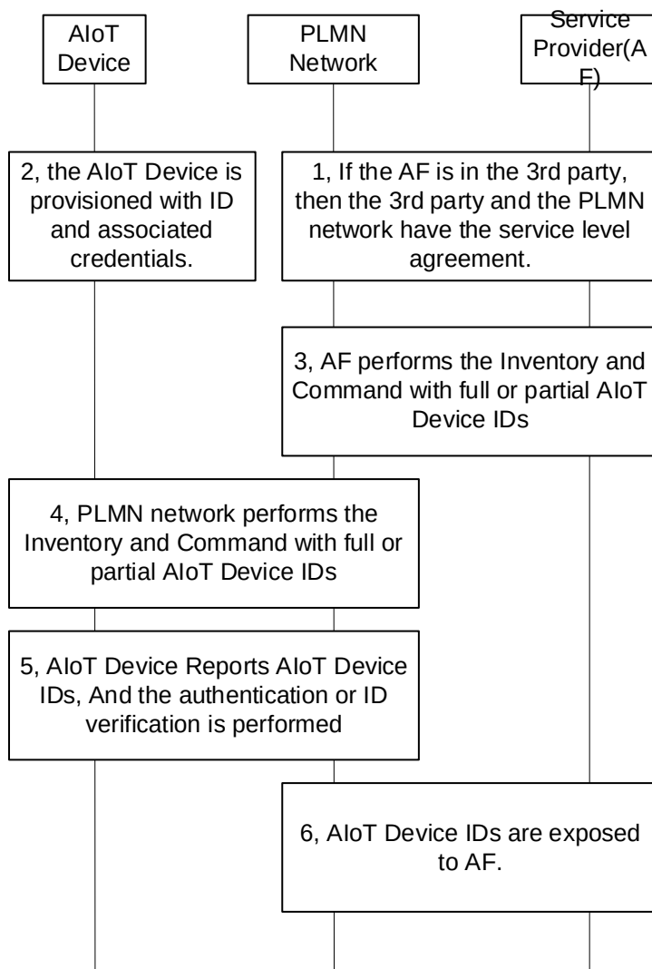
Figure 6.14.2-1: High-level procedure for case 1
