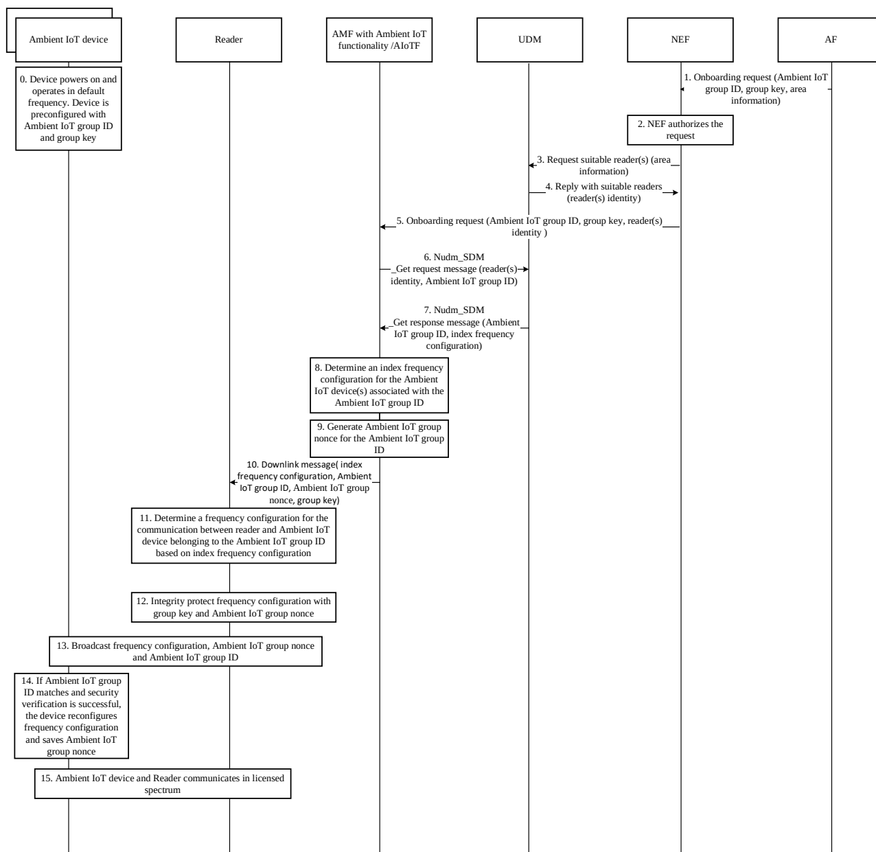
Figure 6.39.2.1-1: Enablement of communication in operator network
