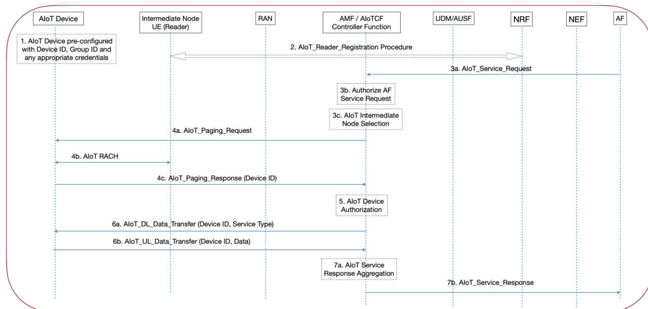
Figure 6.33.2.1-1: AIoT Service Operation Procedure for Type A AIoT Device
