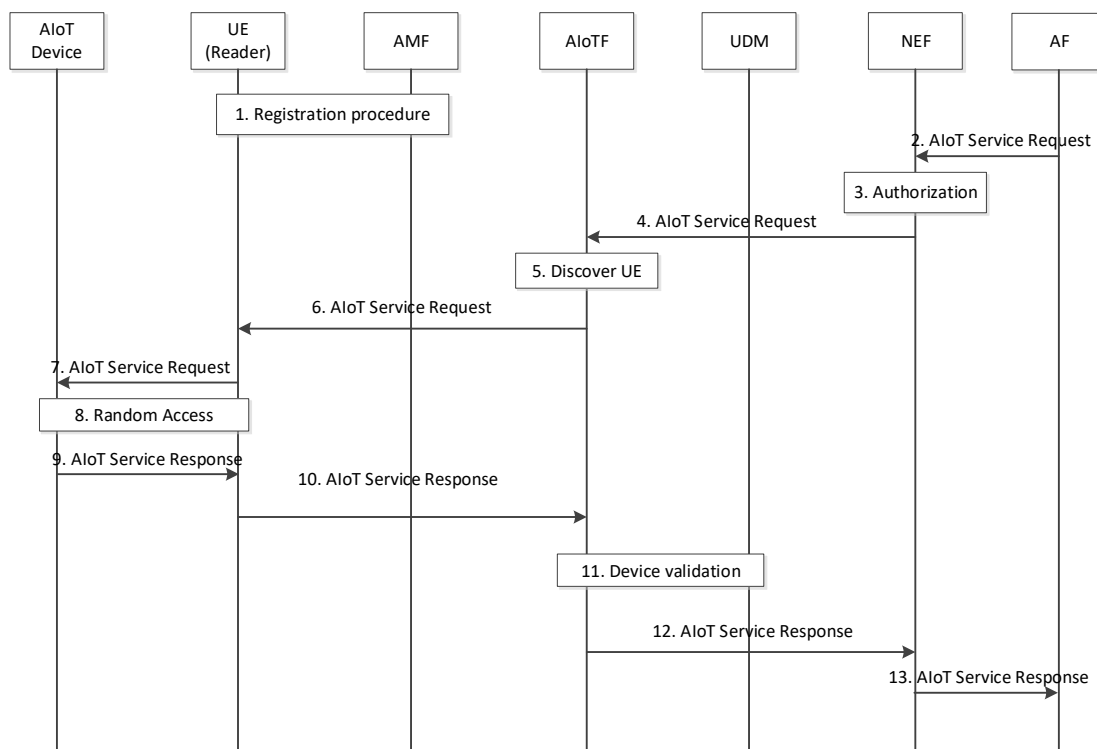
Figure 6.21.2-1: Procedure to support AIoT Services for Topology 2
