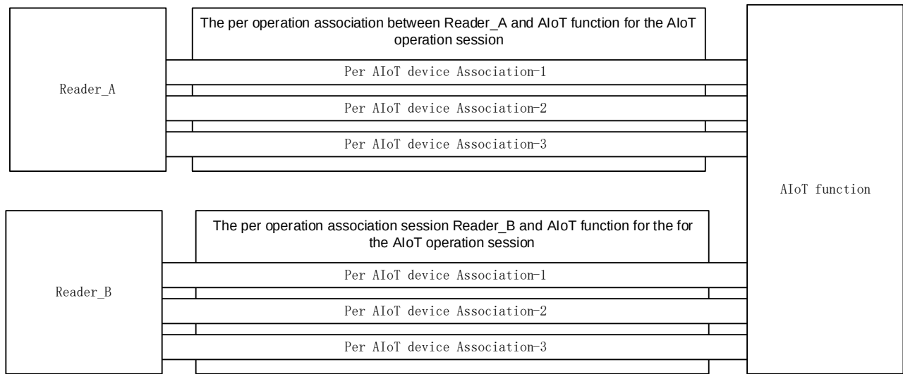
Figure 6.20.1-2: Multiple per AIoT device Association within an AIoT operation
