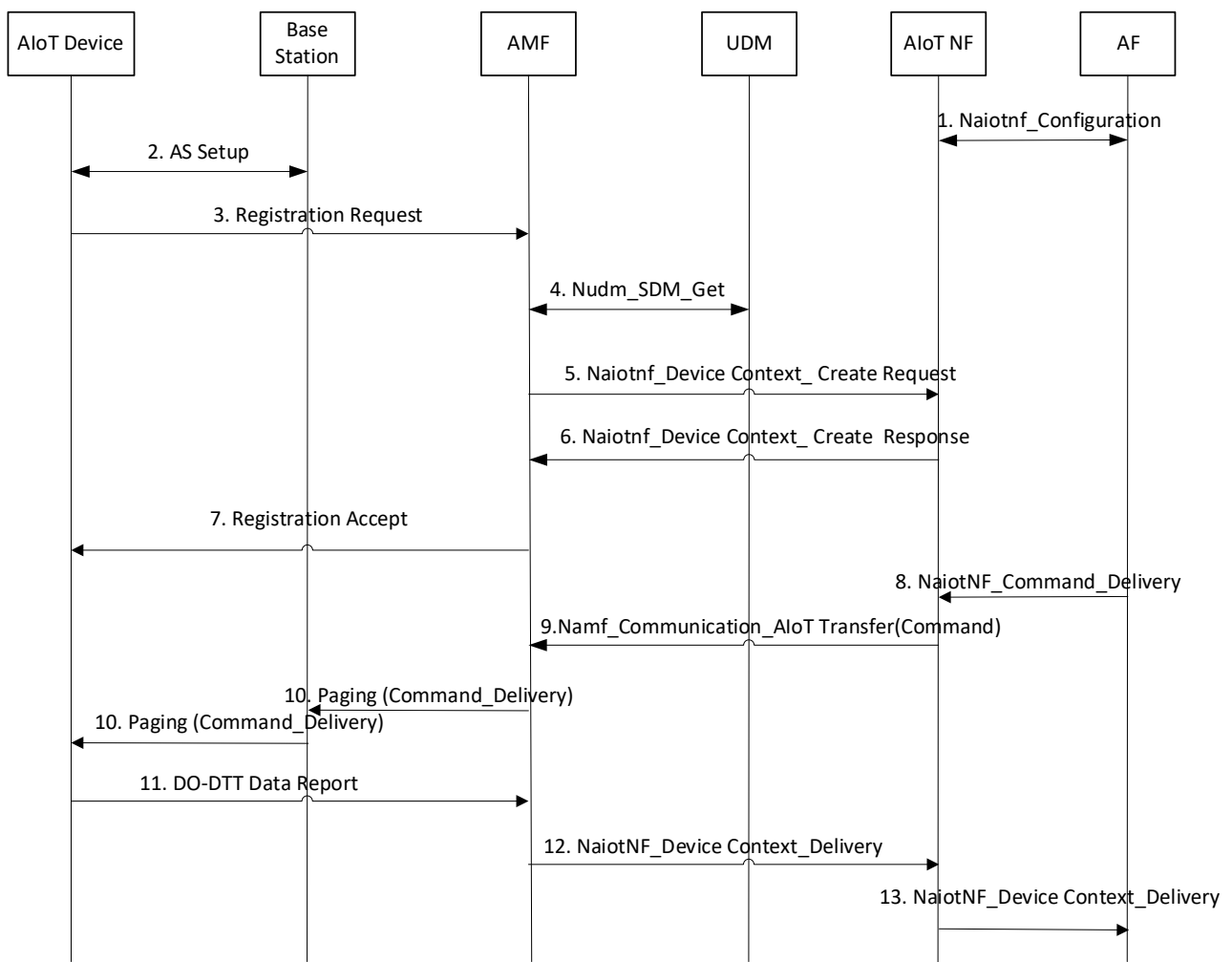
Figure 6.9.2-1 Signalling flow for Information Transfer
