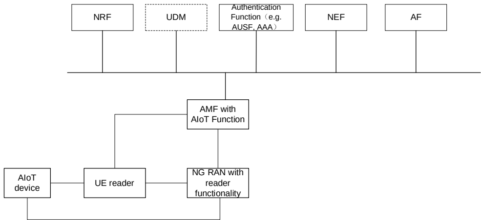
Figure 6.4.1.4.1-1: The example of reference architecture which supporting topology 1 & 2
