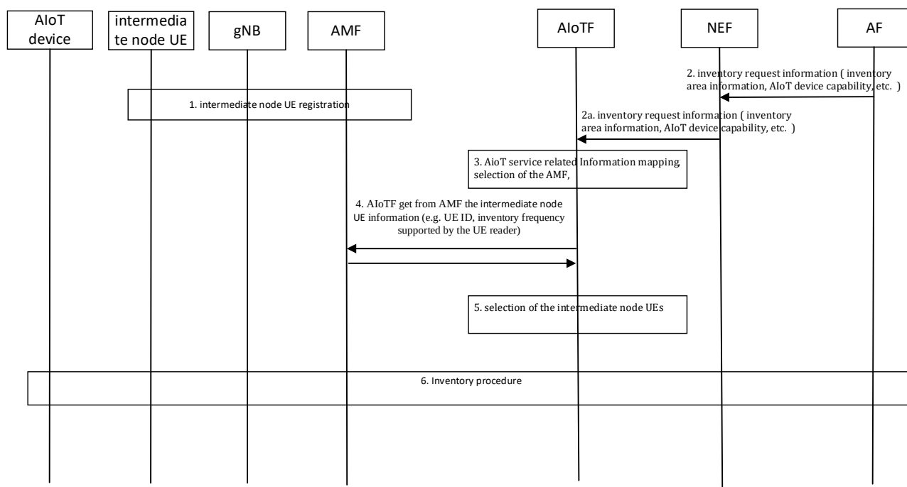
Figure 6.23.2-1: UE reader selection procedure
