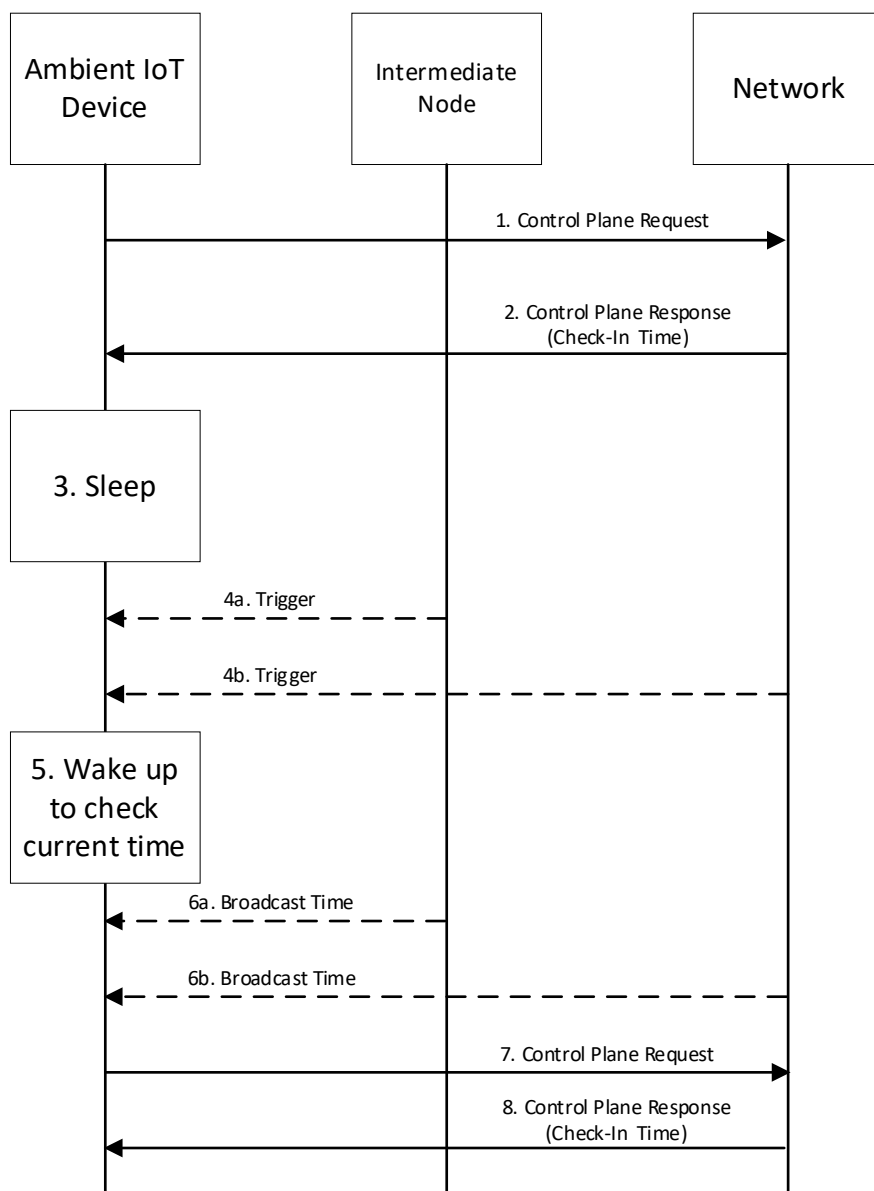
Figure 6.24.2-1: Procedure for Ambient IoT Device Availability Reporting
