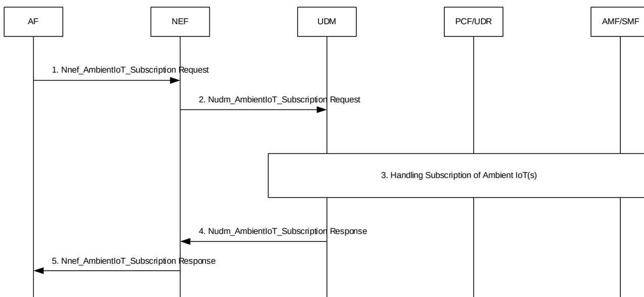
Figure 6.25.2-1: Subscription procedures for Ambient IoT Devices
