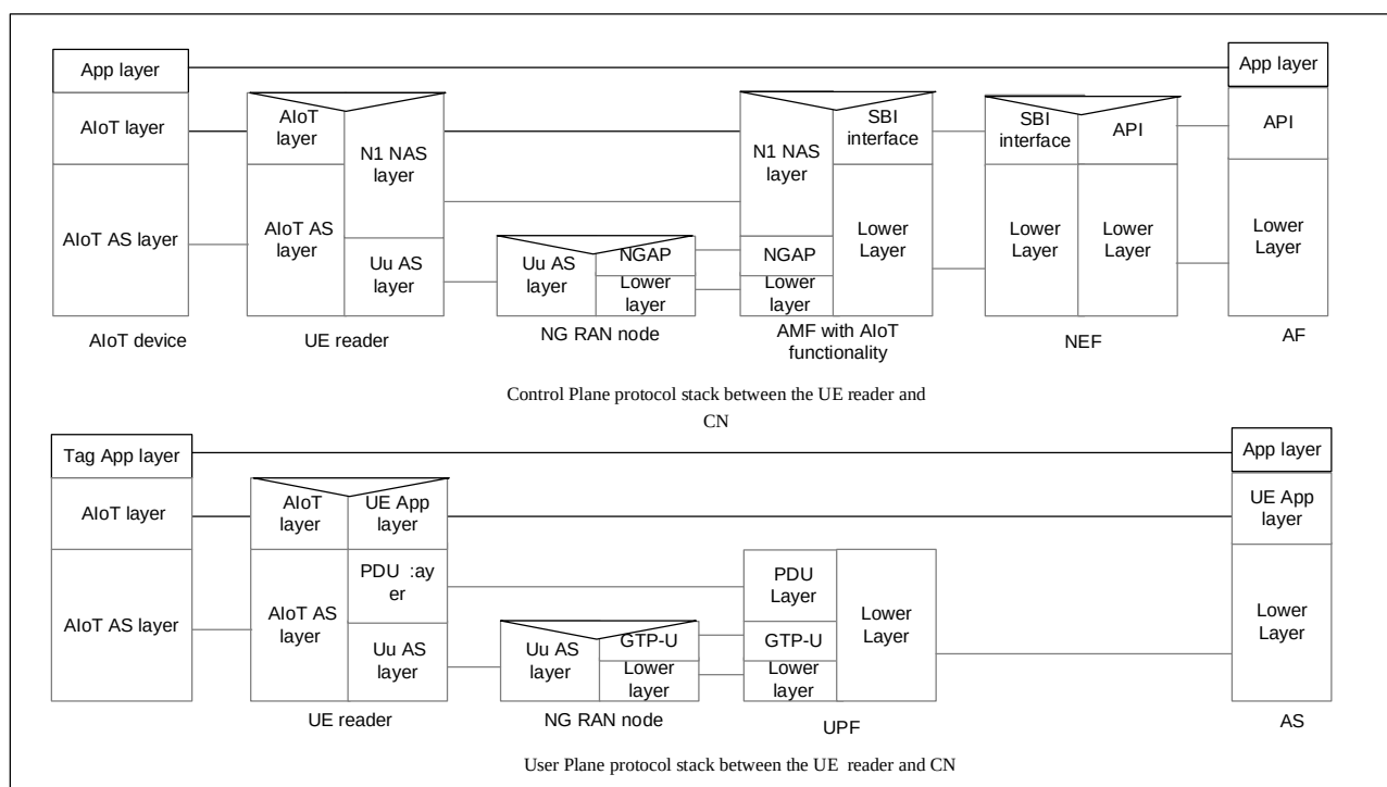
Figure 6.4.1.5-2: Protocol stack example-B for Topology2
