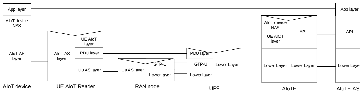
Figure 6.32.2-1: Protocol Stack for AF Based Solution (over user plane)
