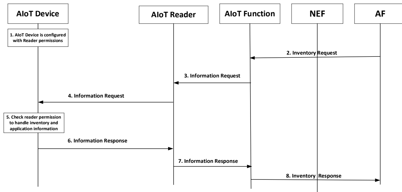
Figure 6.40.2-1: Inventory Procedure where the AIoT Device Checks Reader Permissions before Responding
