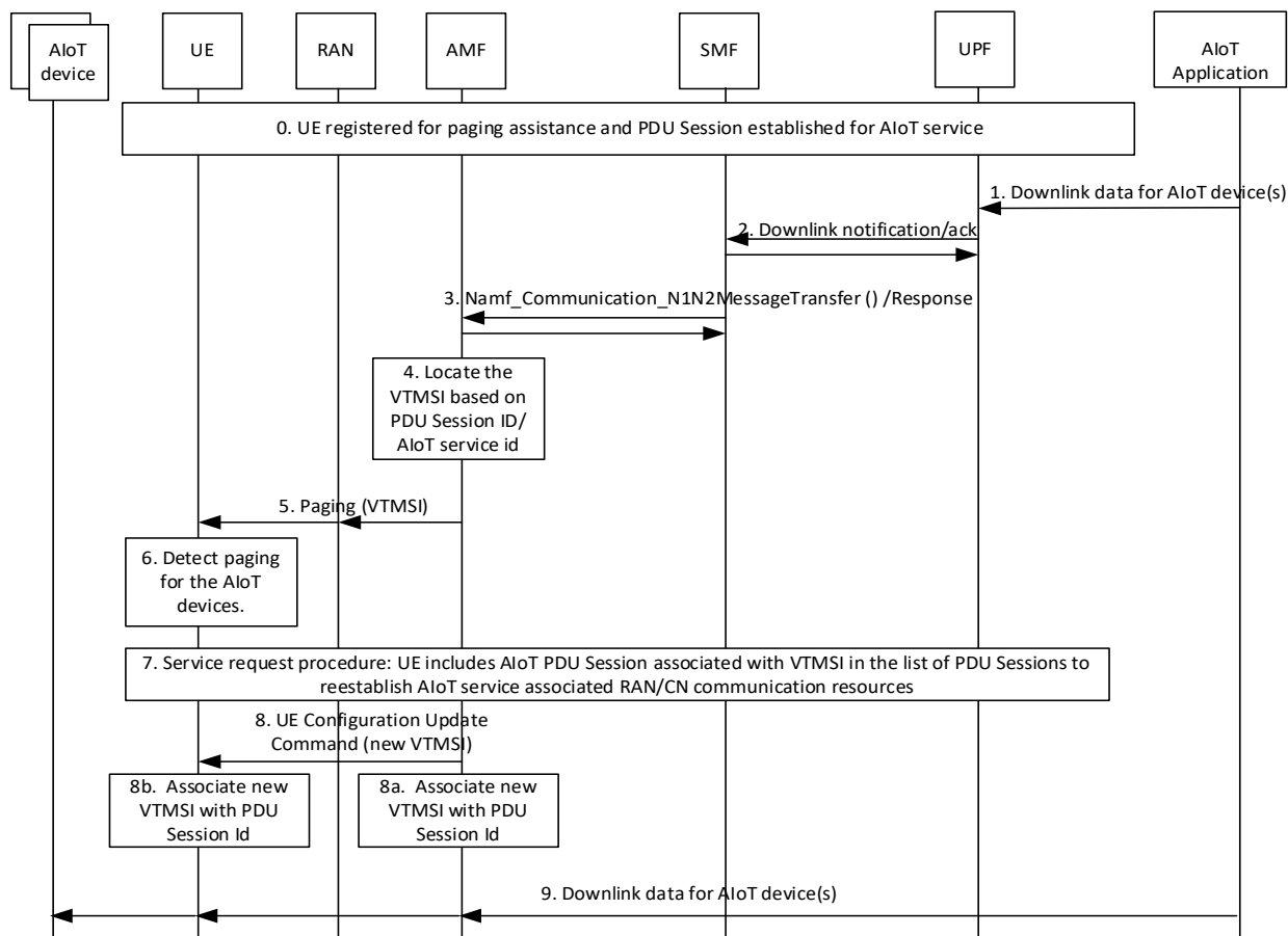
Figure 6.34.2-2: Network triggered service request for UE
