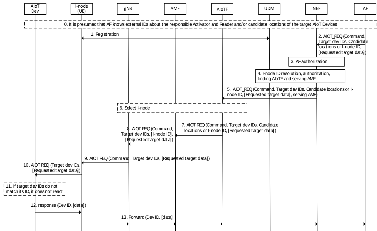
Figure 6.11.2.1-1: Information Flow for AIoT data retrieval
