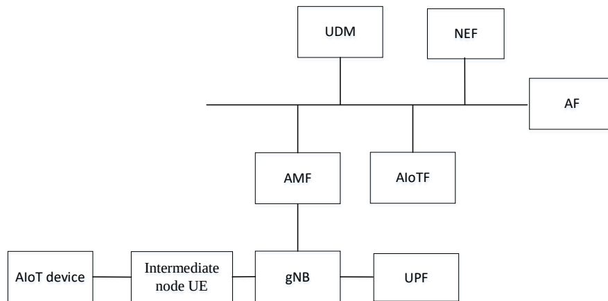
Figure 6.23.1.3-1: Reference architecture
