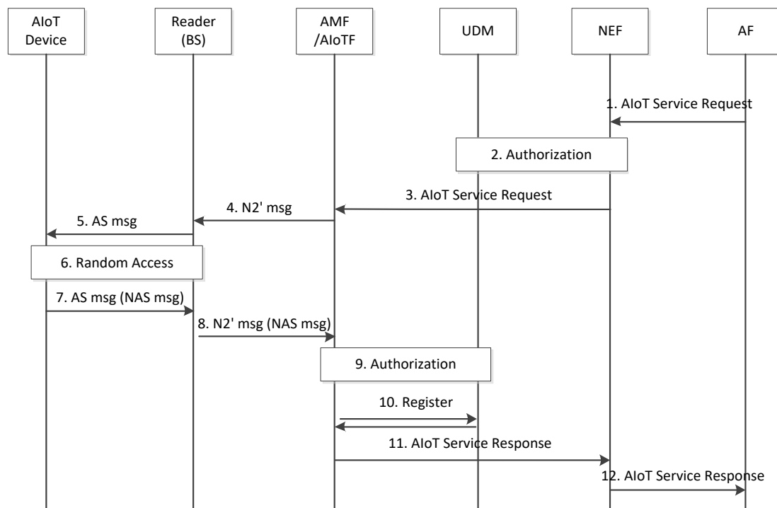
Figure 6.5.2-1: Procedure for NAS-based information transfer for Ambient IoT Services
