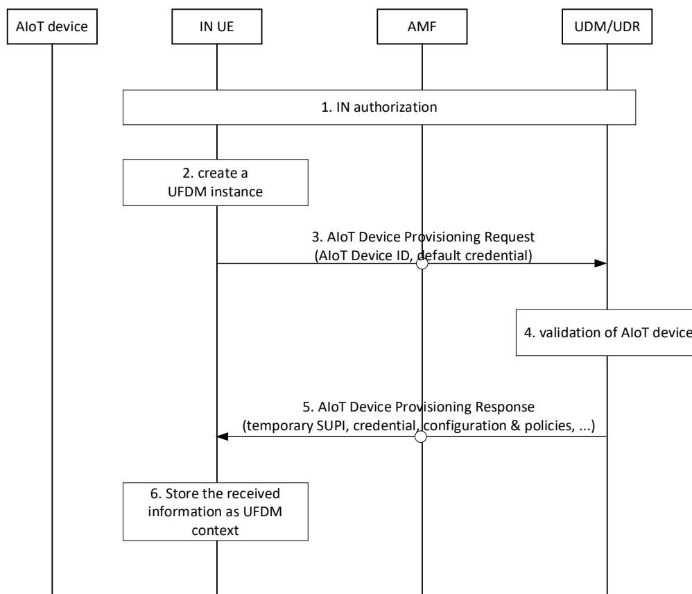
Figure 6.12.2.1-1: UFDm instantiation and provisioning
