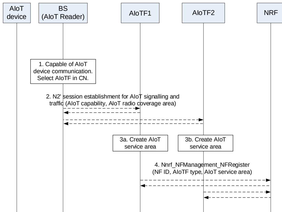
Figure 6.19.3.1-1: Signalling flow of the N2' association establishment between of AIoT capable BS node and AIoTF
