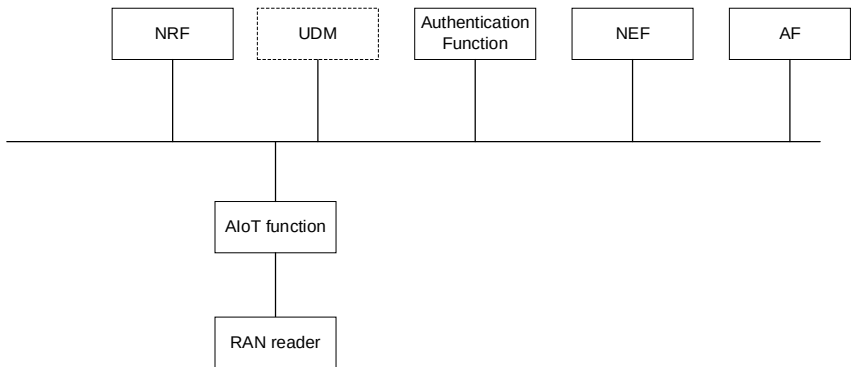
Figure 6.4.1.4.1-2: The example of reference architecture for alternative 1
