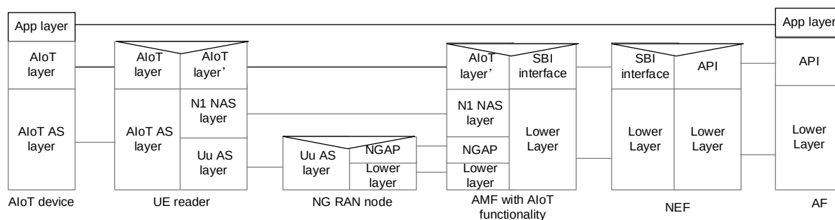
Figure 6.4.1.5-2: protocol stack example-A for Topology2
