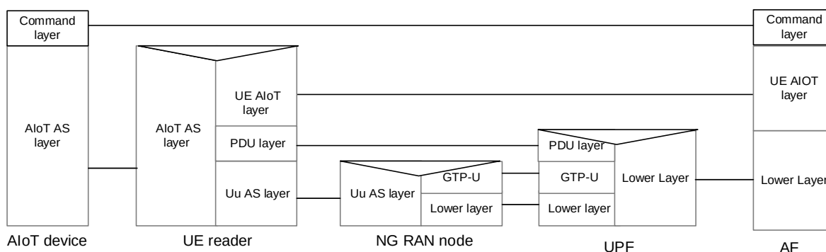
Figure 6.22.1.2-1: Protocol Stack for AF Based Solution (over user plane)
