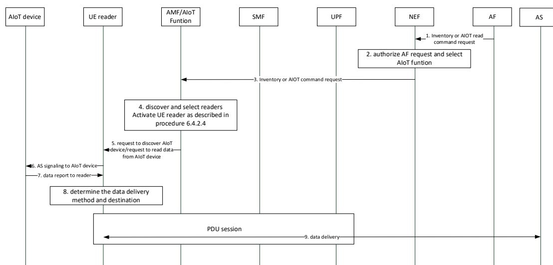
Figure 6.4.2.3-1: Procedure flow of user plane data delivery for multiple AIoT devices
