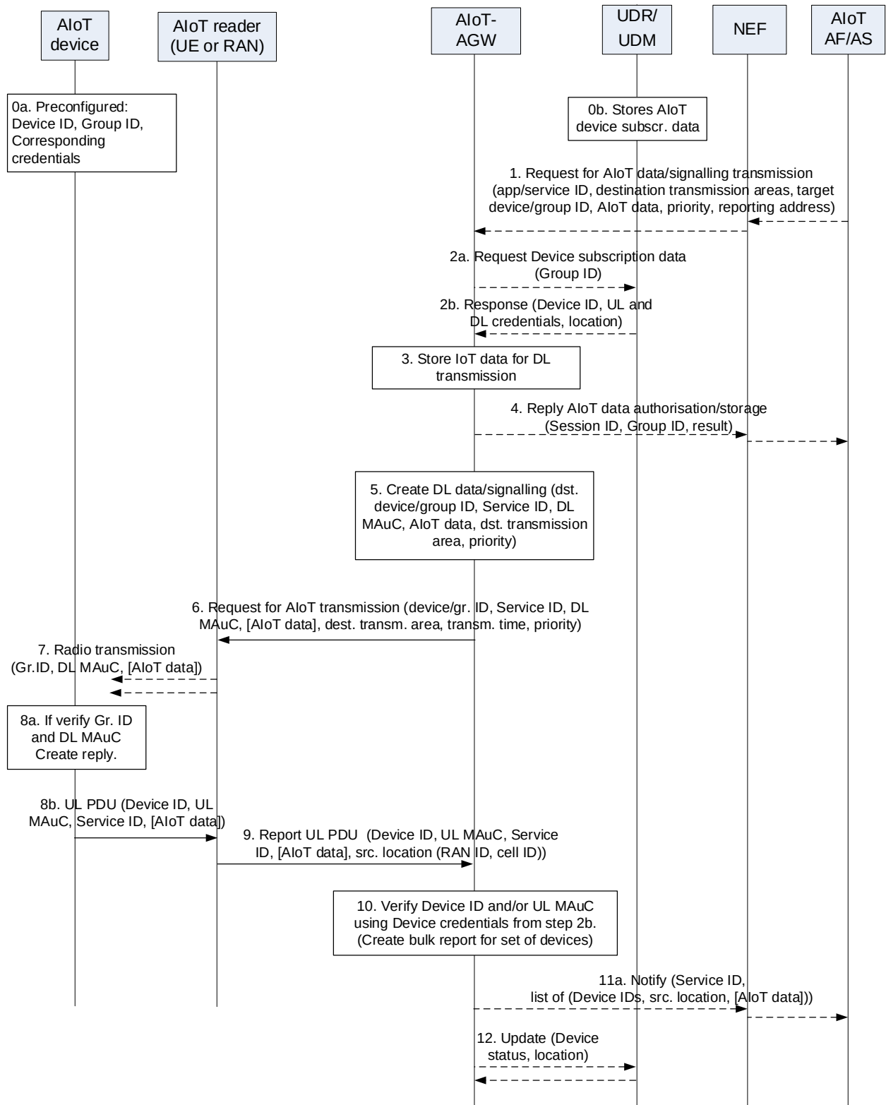
Figure 6.6.3.1-1: Signalling flow for the authentication and ID validation of AIoT devices and secure AIoT communication
