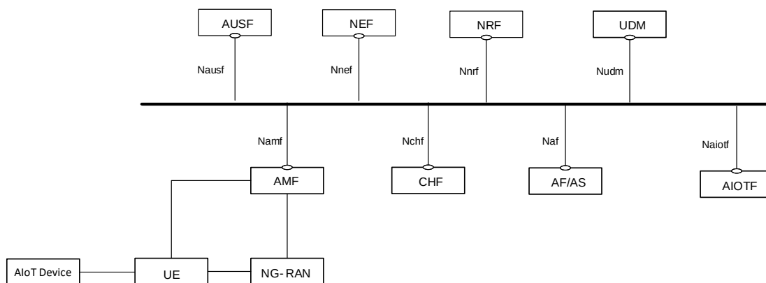
Figure 6.30.1.1-1: System Architecture of Supporting AIoT Devices using AIOTF for Topology 2
