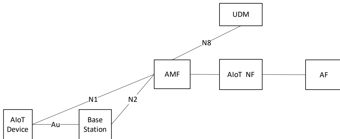
Figure 6.9.1-1 5GS enhancement to support AIoT Devices
