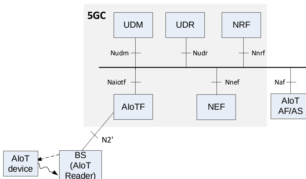
Figure 6.19.2-1: Assumed architecture for topology 1
