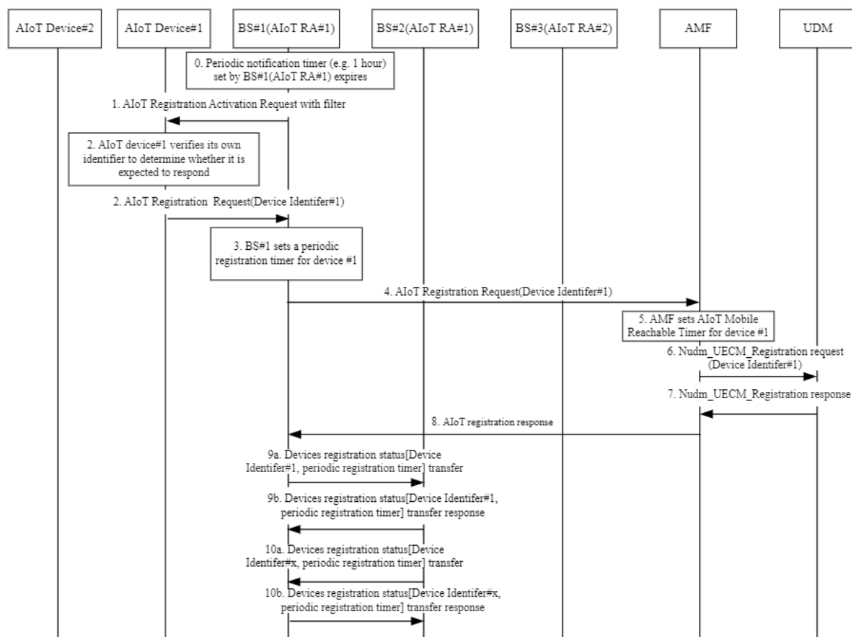
Figure 6.29.2.1-1: Periodic triggered AIoT devices to perform Registration Update
