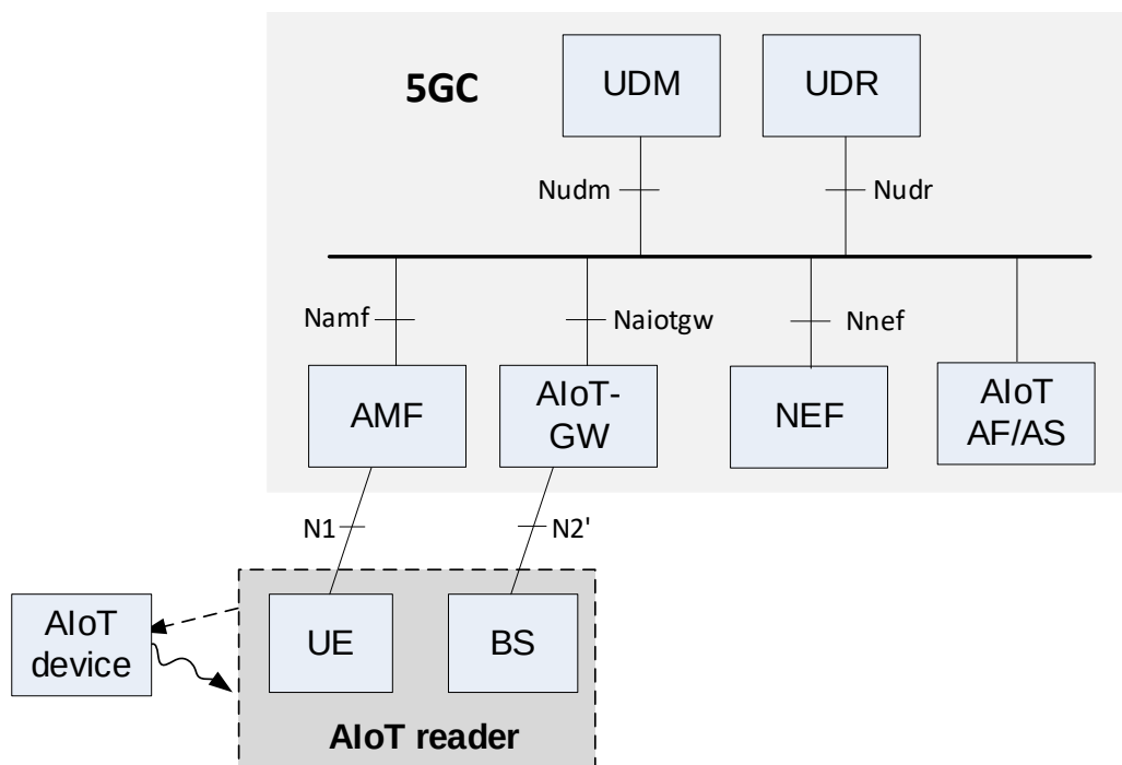
Figure 6.6.2-1: Assumed architecture for AIoT device authentication and AIoT communication
