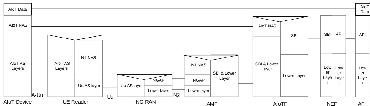
Figure 6.21.1-2: Protocol stack to support AIoT Services for Topology 2
