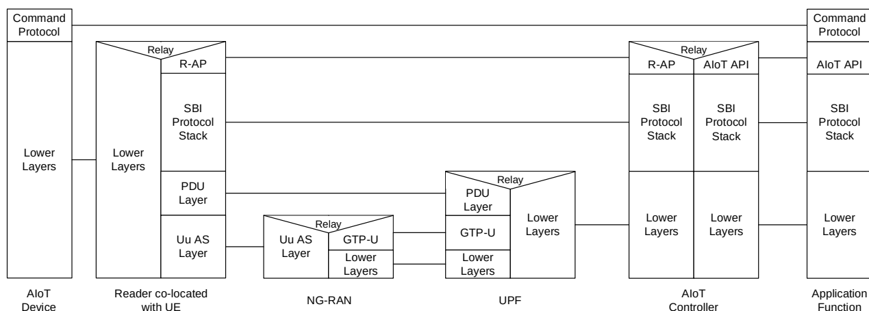
Figure 6.3.1.6.2-2: Protocol stack between AIoT Device and Application Function for Topology 2
