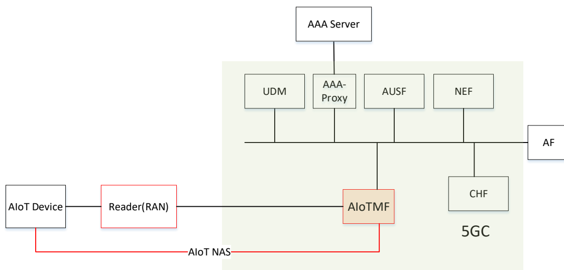
Figure 6.17.1.2-1: 5GC enhancements to support Ambient IoT for topology 1
