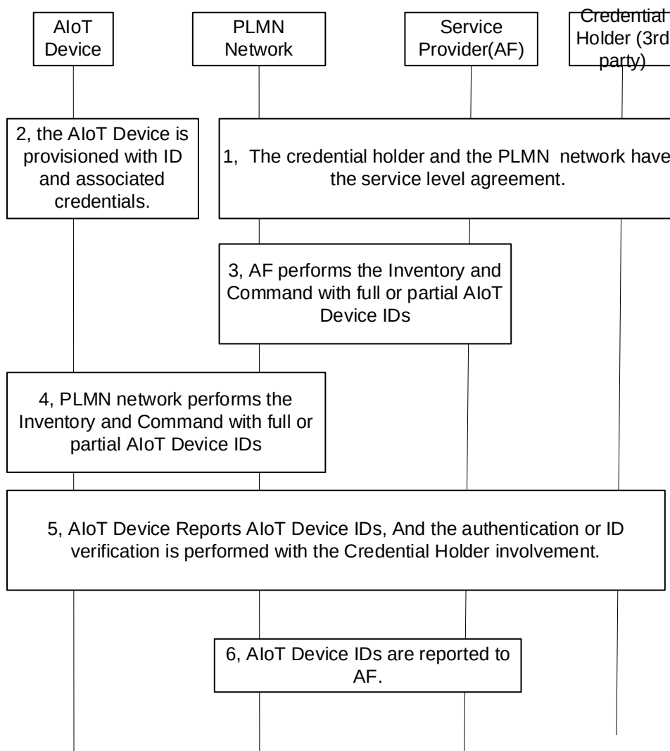
Figure 6.14.2-2: High-level procedure for case 2
