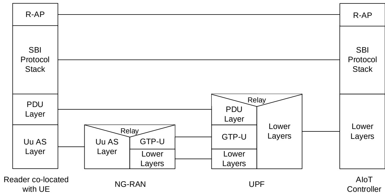
Figure 6.3.1.6.1-2: Control Plane between Reader and AIoT Controller for Topology 2 using a PDU Session between UE and UPF
