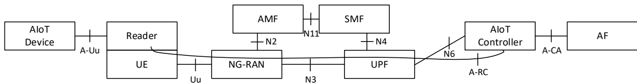
Figure 6.3.1.4-2: Ambient IoT system architecture for Topology 2
