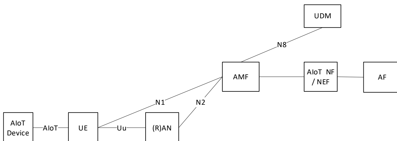
Figure 6.11.1-1 5GS enhancement to support AIoT Devices for Topology 2
