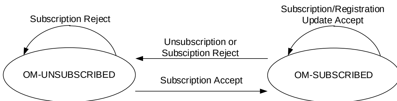
Figure 6.25.1-2: Online-subscription Management state model in AF and UDM
