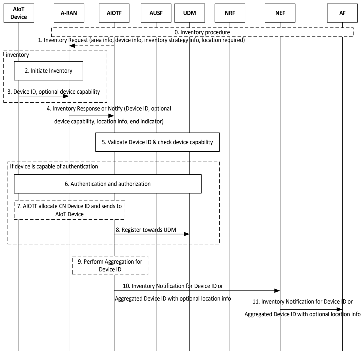
Figure 6.8.2.2-1: Periodic Inventory Procedure
