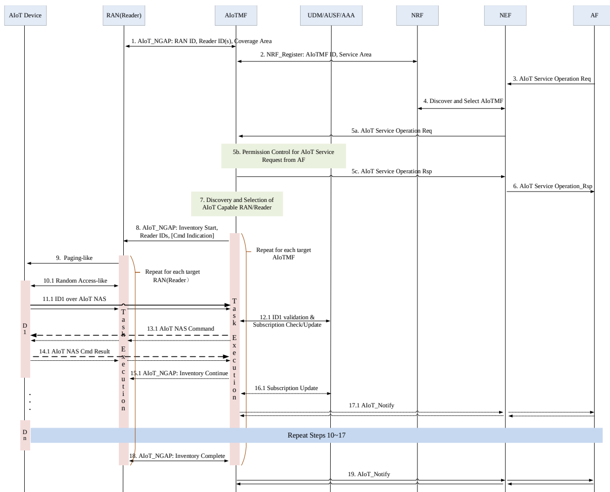
Figure 6.17.2.2-1: AIoT Service High-Level Information Flow
