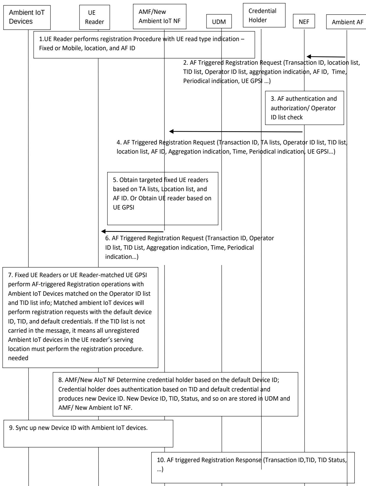
Figure 6.10.2-2: AF triggered Registration Procedure for Topology 2
