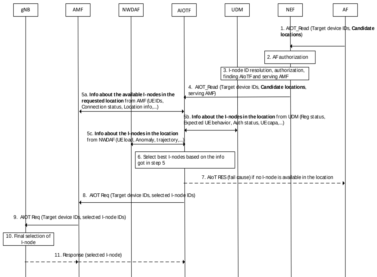
Figure 6.11.2.2-1: Information Flow for selecting I-node based on location of target devices from AF
