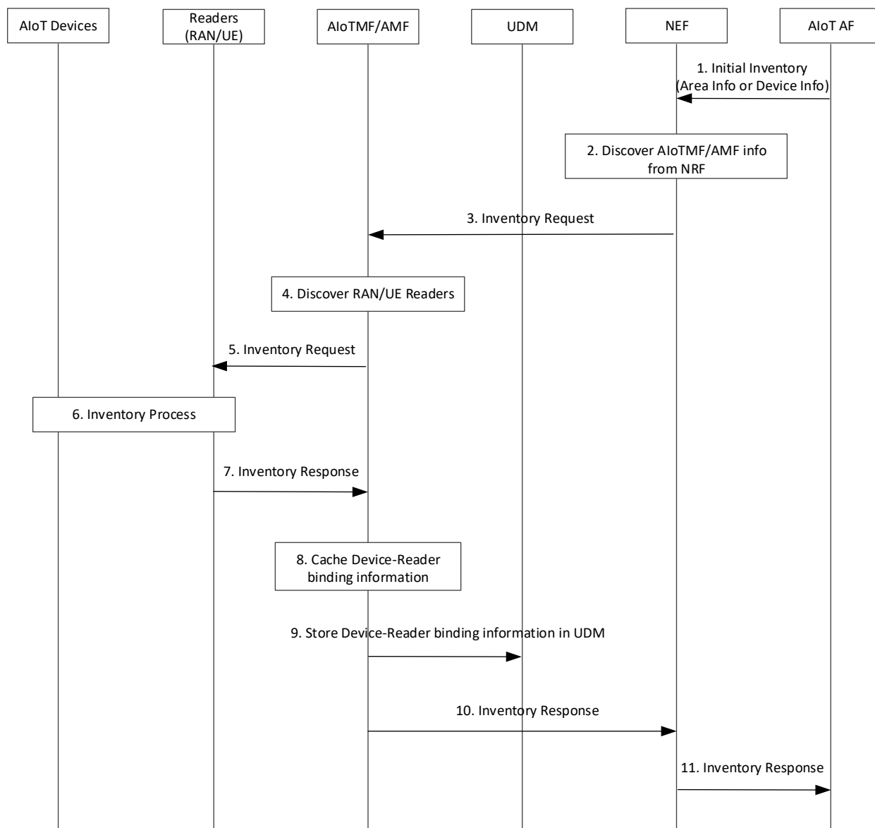
Figure 6.28.2.1-1: Device-Reader binding information storage
