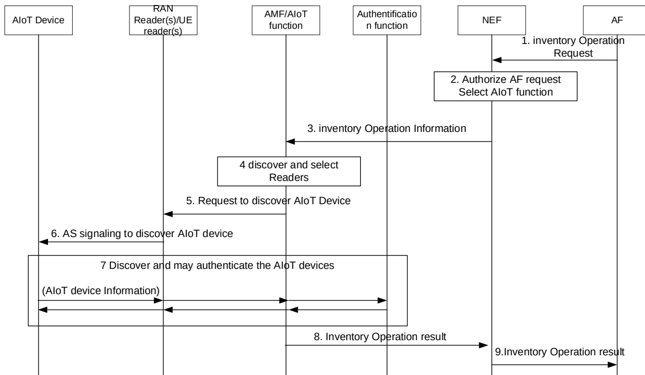
Figure 6.4.2.1-1: Inventory Service Flow
