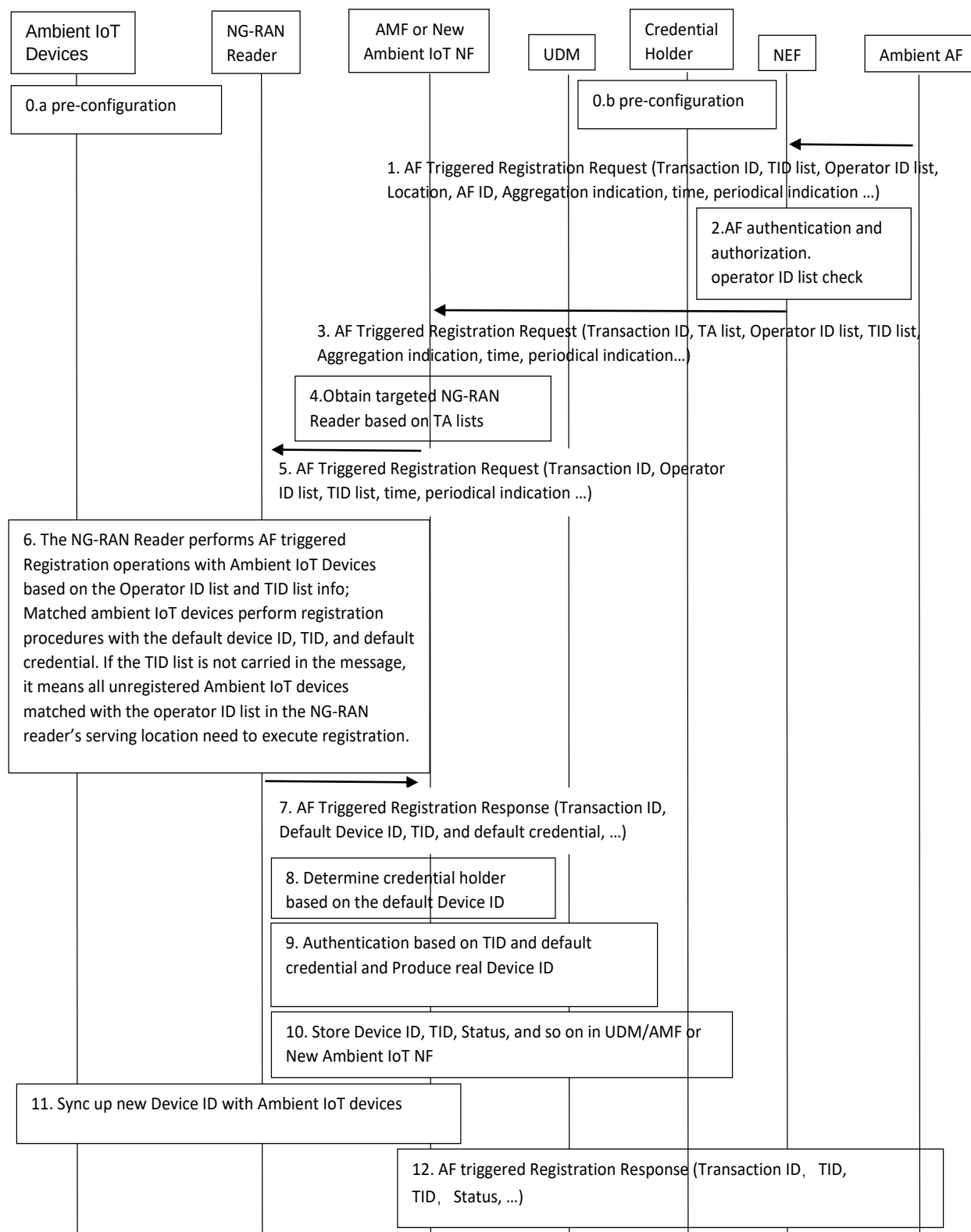
Figure 6.10.2-1: AF triggered Registration Procedure for Topology 1
