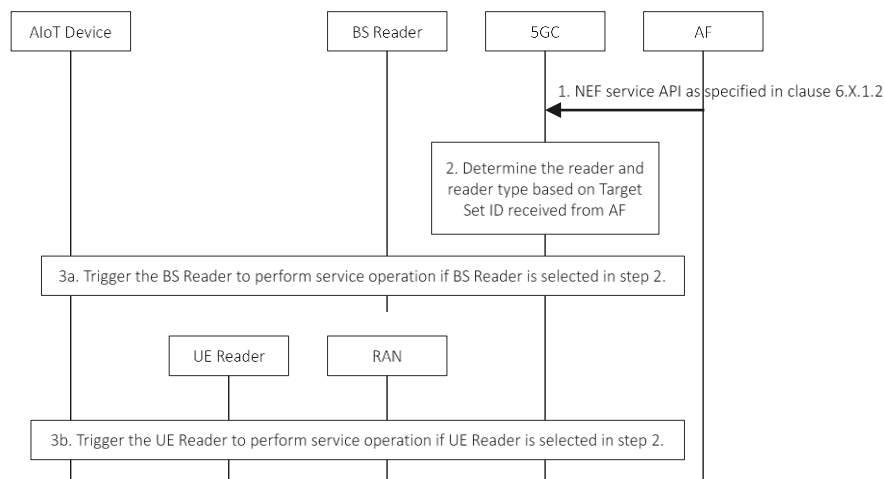
Figure 6.26.2-1: Procedure for unified API between 5GC and AF to support AIoT service
