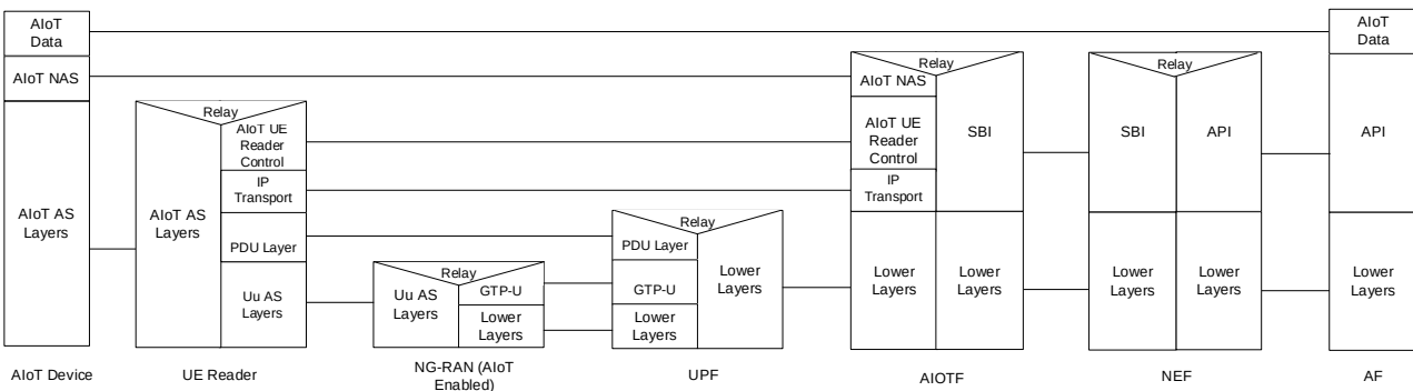
Figure 8.1.3.2-2: Protocol stack for the user-plane architecture for Topology 2
