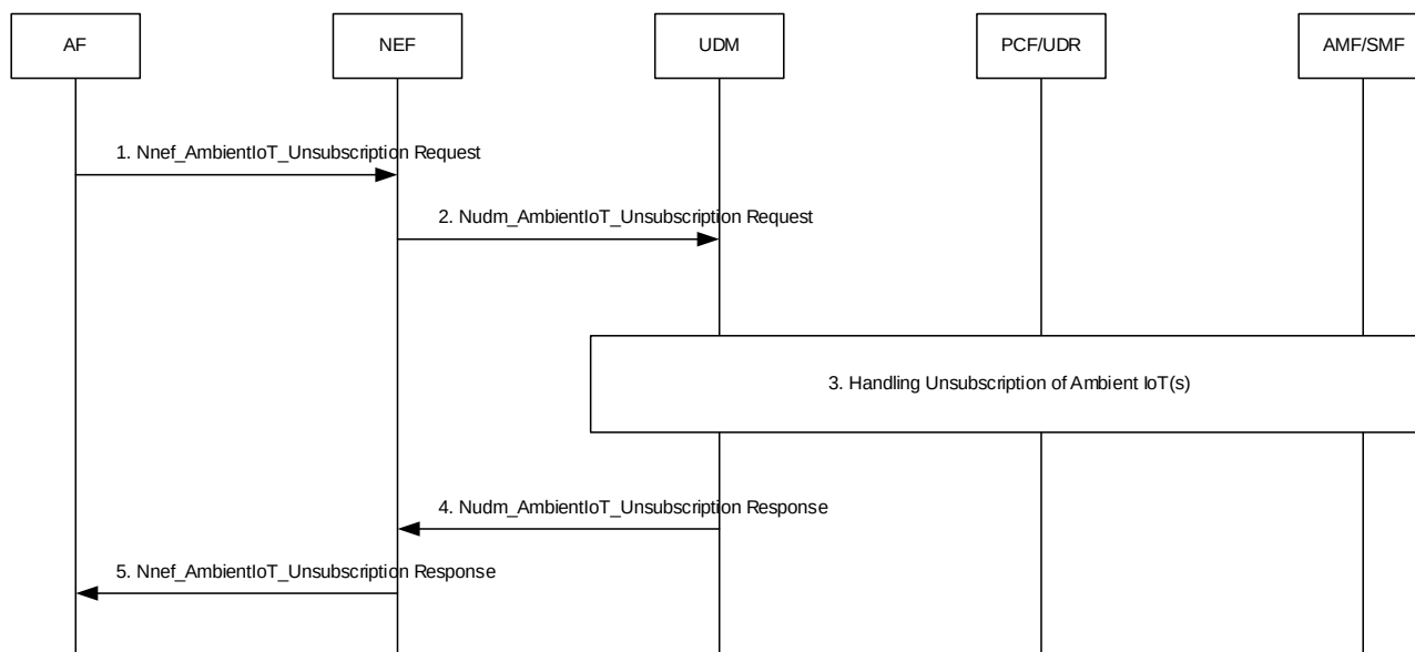
Figure 6.25.2-2: Unsubscription procedures for Ambient IoT Devices
