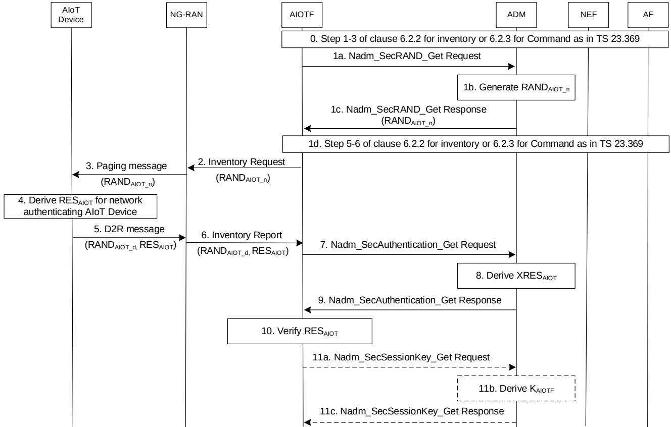
Figure 5.2.2-1: Authentication procedure
